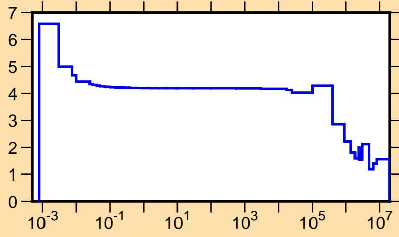
\sigma vs. E for ^{13}\text{C}(n,\text{tot.})
