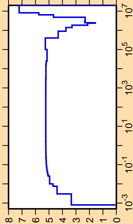
\Delta\sigma/\sigma vs. E for ^{13}\text{C}(n,\text{el.})
