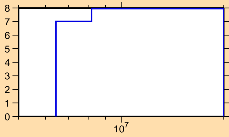
\Delta\sigma/\sigma vs. E for ^{13}\text{C}(n,\text{nonel.})
