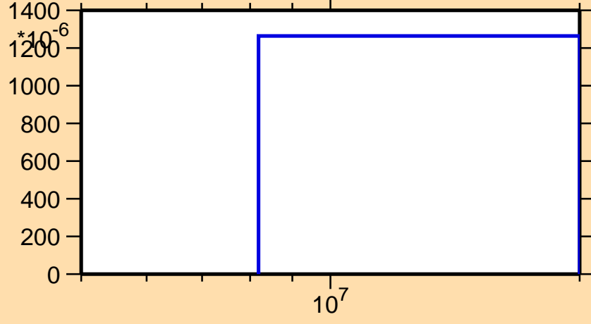
\sigma vs. E for ^{13}\text{C}(n,p)
