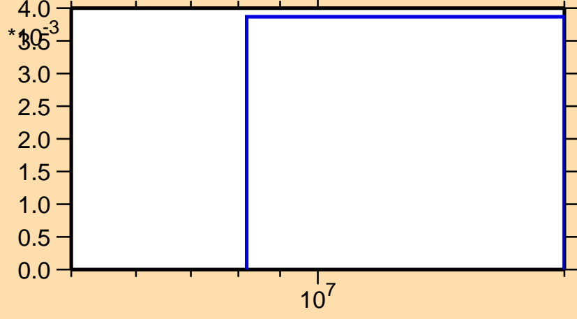
\sigma vs. E for ^{13}\text{C}(n,2n)
