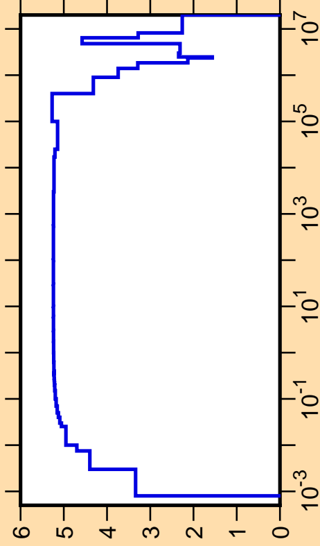
\Delta\sigma/\sigma vs. E for ^{13}\text{C}(n,\text{tot.})
