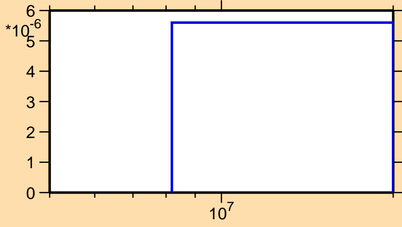
\sigma vs. E for ^{13}\text{C}(n,2n\alpha)
