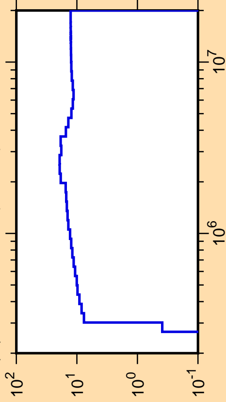
\Delta\mu/\mu vs. E for ^{14}\text{C}(\text{mt251})
