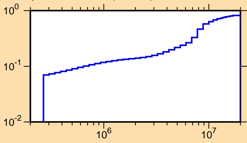
\mu vs. E for ^{14}\text{C}(\text{mt251})
