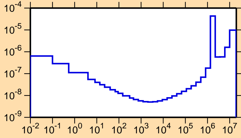
\sigma vs. E for ^{14}\text{C}(n,\gamma)
