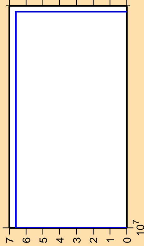
\Delta\sigma/\sigma vs. E for ^{14}\text{C}(n,3n)
