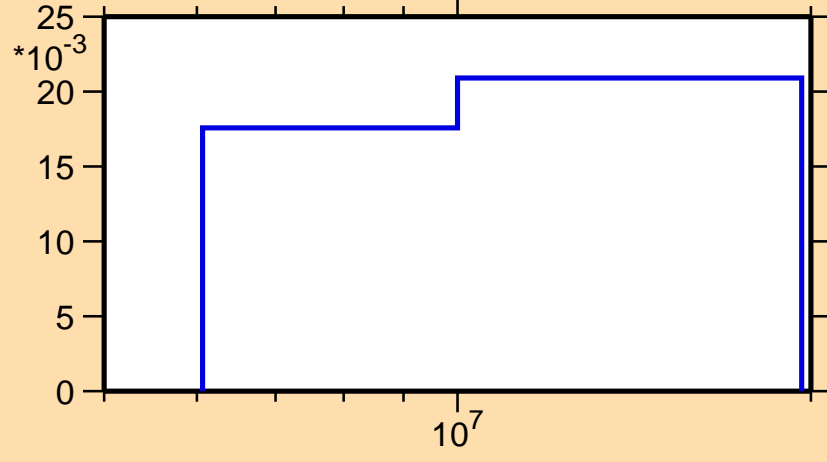
\sigma vs. E for ^{14}\text{C}(n,n_2)
