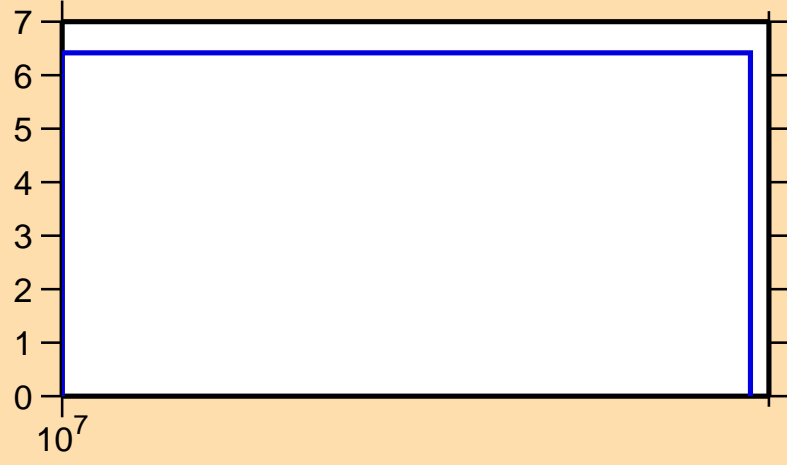
\Delta\sigma/\sigma vs. E for ^{14}\text{C}(n,el.)
