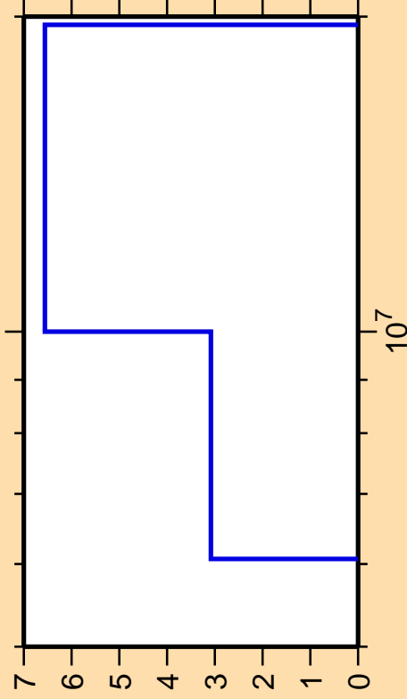
\Delta\sigma/\sigma vs. E for ^{14}\text{C}(n,n_2)
