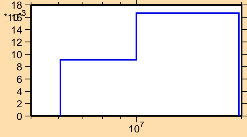
\sigma vs. E for ^{14}\text{C}(n,n_4)
