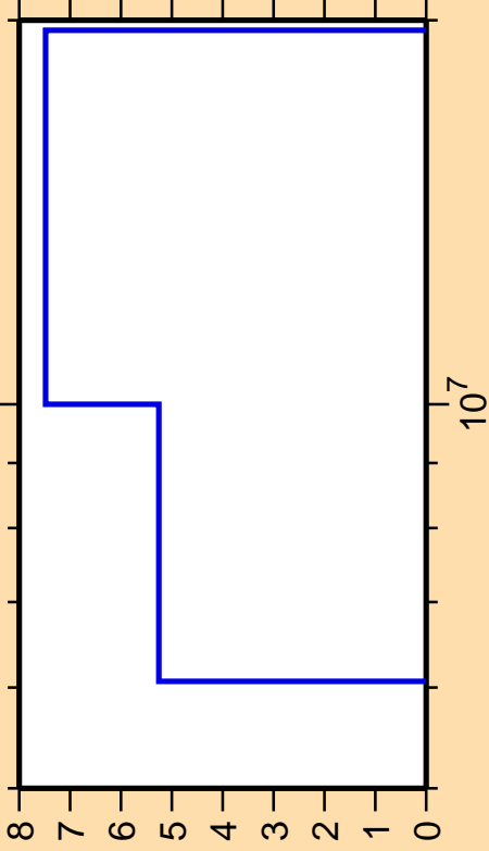
\Delta\sigma/\sigma vs. E for ^{14}\text{C}(n,n_1)
