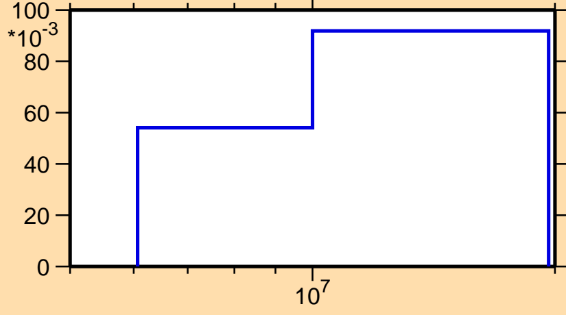
\sigma vs. E for ^{14}\text{C}(n,n_3)
