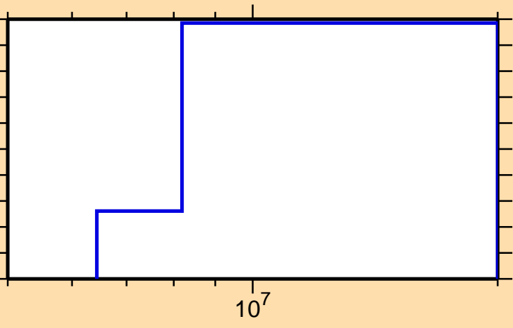
\sigma vs. E for ^{14}\text{C}(n,n_4)
