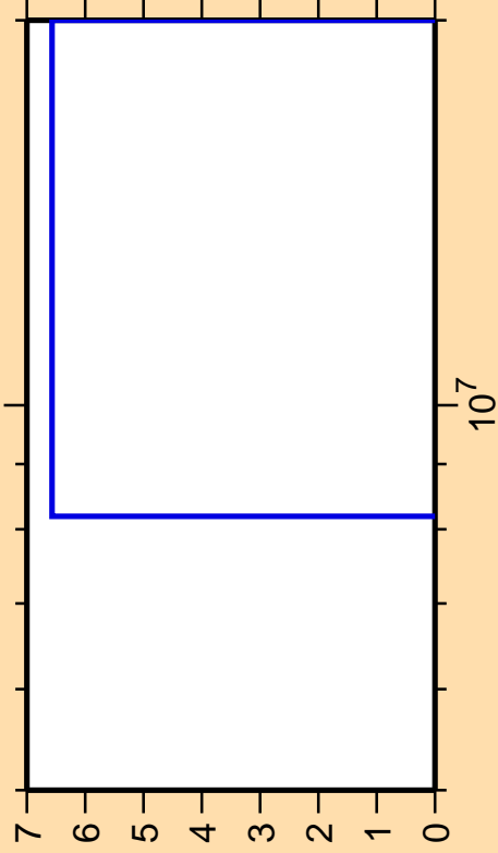
\Delta\sigma/\sigma vs. E for ^{14}\text{C}(n,n_1)
