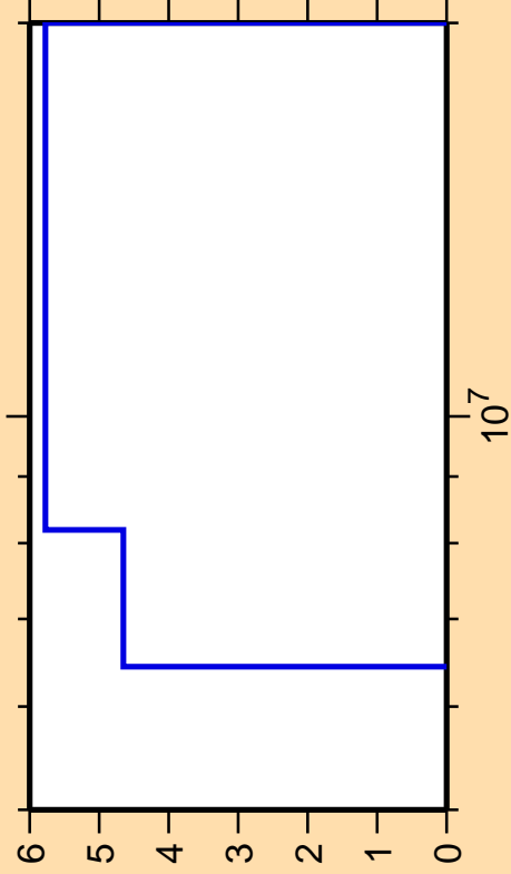
\Delta\sigma/\sigma vs. E for ^{14}\text{C}(n,\text{inel.})
