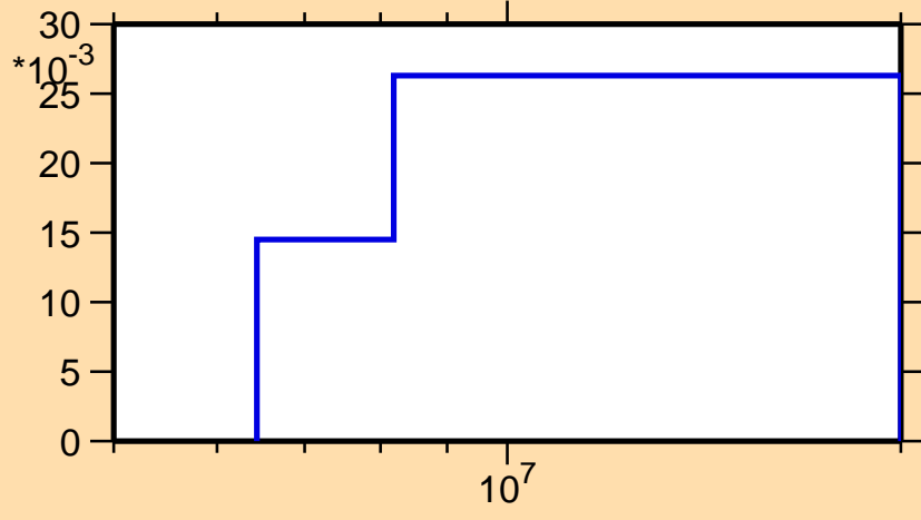
\sigma vs. E for ^{14}\text{C}(n,n_2)
