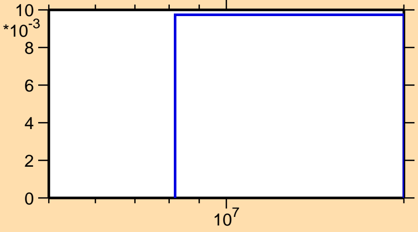
\sigma vs. E for ^{14}\text{C}(n,\alpha)
