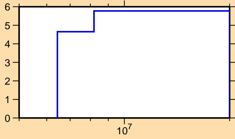
\Delta\sigma/\sigma vs. E for ^{14}\text{C}(n,\text{inel.})
