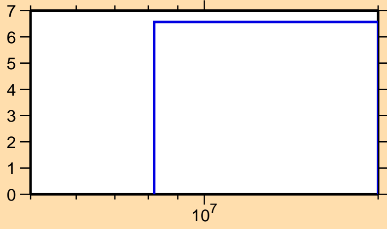
\Delta\sigma/\sigma vs. E for ^{14}\text{C}(n,n_1)
