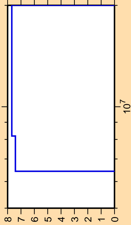
\Delta\sigma/\sigma vs. E for ^{14}\text{C}(n,n_4)
