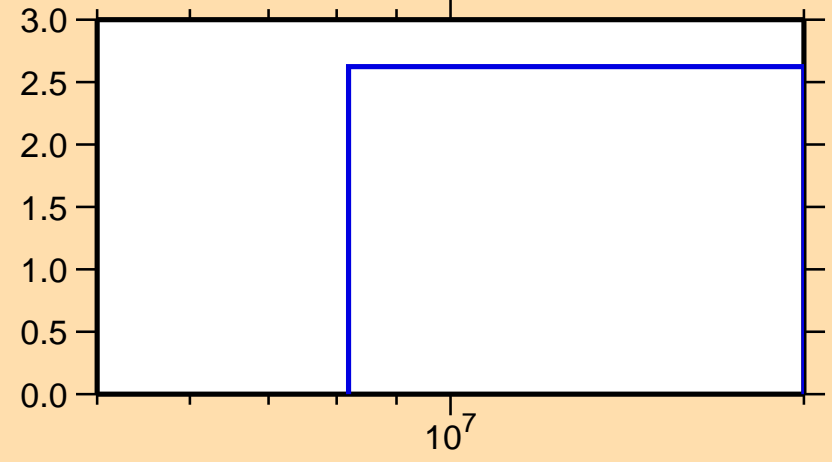
\Delta\sigma/\sigma vs. E for ^{14}\text{C}(n,\text{tot.})
