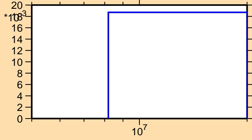
\sigma vs. E for ^{14}\text{C}(n,2n)
