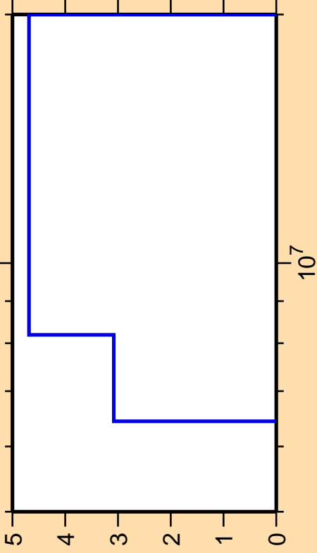
\Delta\sigma/\sigma vs. E for ^{14}\text{C}(n,n_2)
