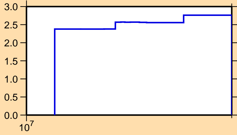
\Delta\sigma/\sigma vs. E for ^{15}\text{C}(n,tot.)
