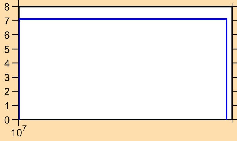
\Delta\sigma/\sigma vs. E for ^{15}\text{C}(n,p)
