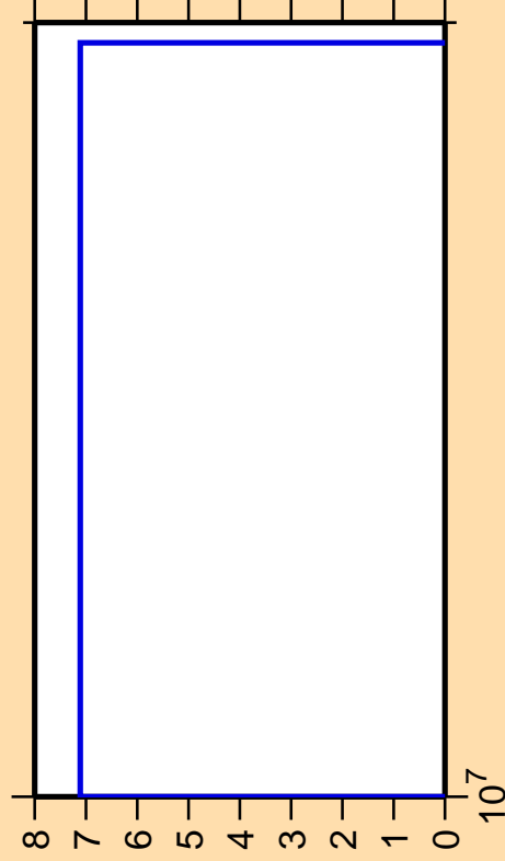
\Delta\sigma/\sigma vs. E for ^{15}\text{C}(n,p)
