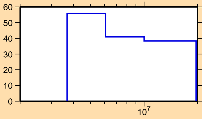
\Delta\sigma/\sigma vs. E for ^{41}\text{Ca}(n,ncont.)
