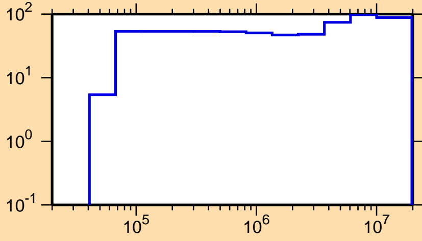
\Delta\sigma/\sigma vs. E for ^{41}\text{Ca}(n,\gamma)
