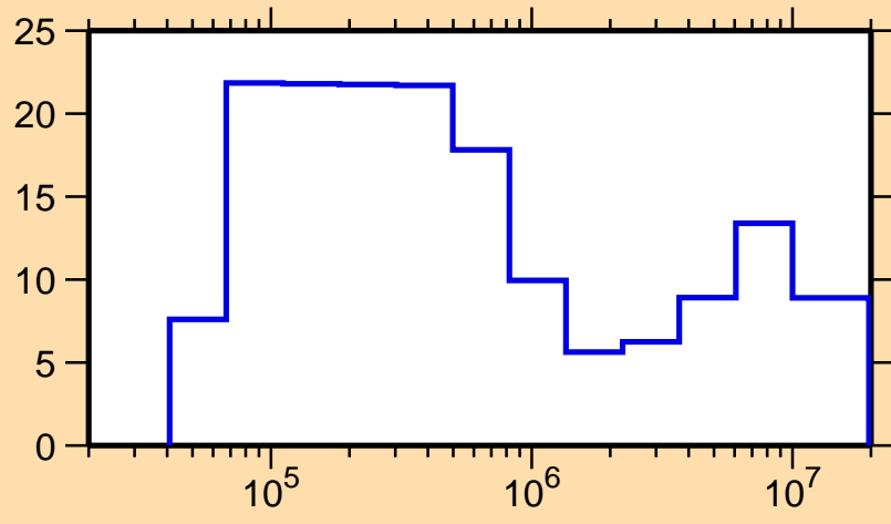
\Delta\sigma/\sigma vs. E for ^{41}\text{Ca}(n,el.)
