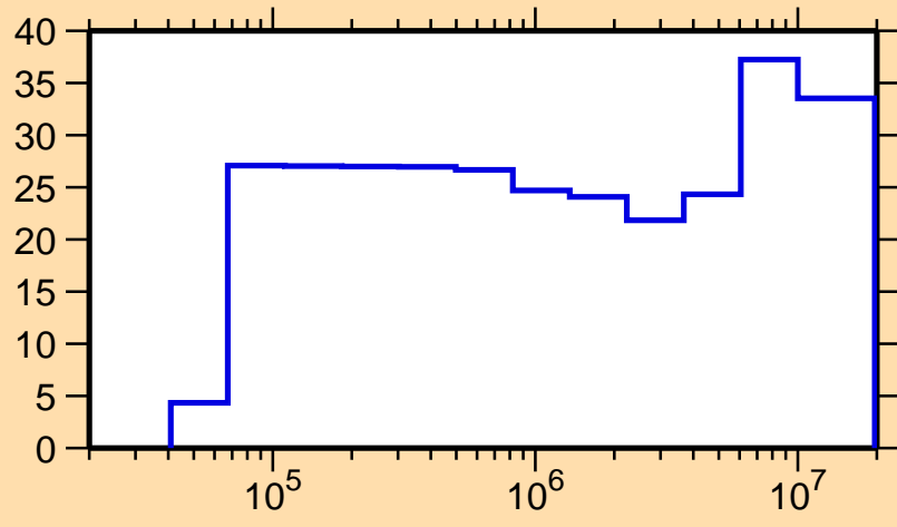
\Delta\sigma/\sigma vs. E for ^{41}\text{Ca}(n,p)
