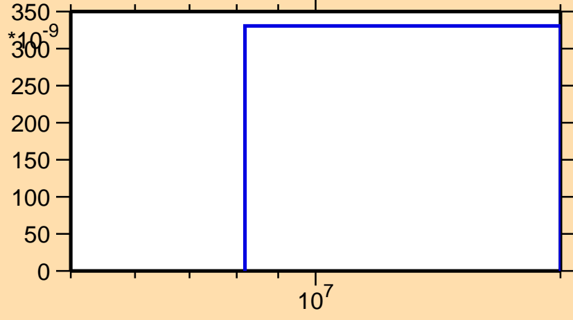
\sigma vs. E for ^{41}\text{Ca}(n,2np)
