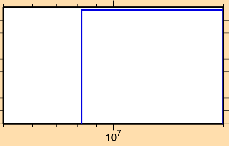
\sigma vs. E for ^{41}\text{Ca}(n,\text{nd})
