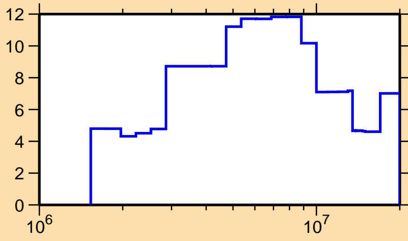
\Delta\sigma/\sigma vs. E for ^{42}\text{Ca}(n,\text{el.})
