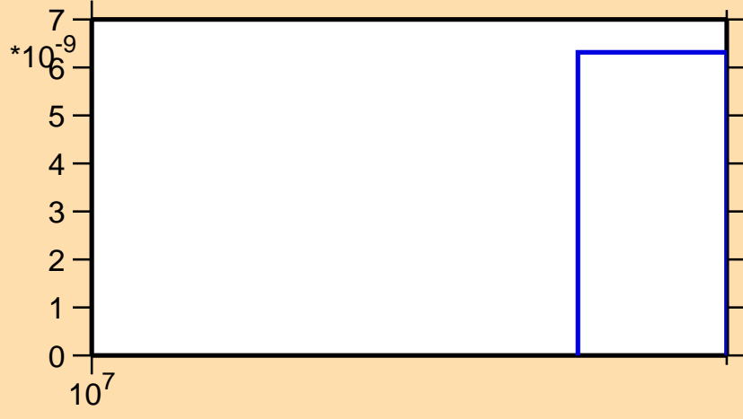
\sigma vs. E for ^{42}\text{Ca}(n,\text{nd})
