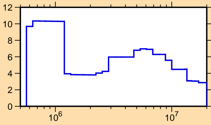
\Delta\sigma/\sigma vs. E for ^{42}\text{Ca}(n,\text{tot.})
