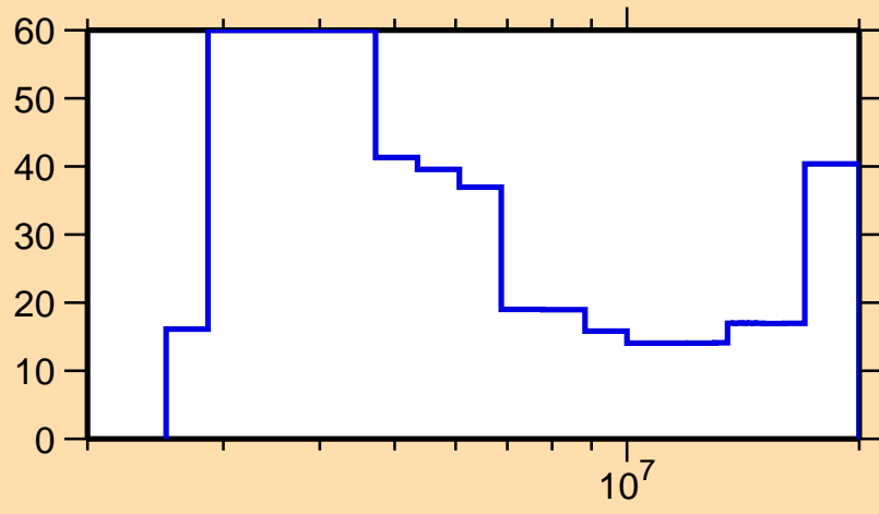
\Delta\sigma/\sigma vs. E for ^{42}\text{Ca}(n,p)
