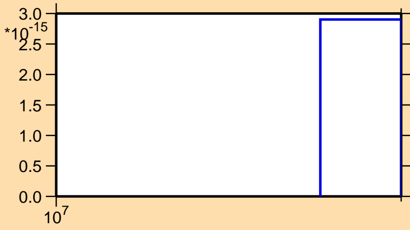
\sigma vs. E for ^{42}\text{Ca}(n,2n\alpha)
