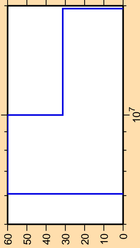
\Delta\sigma/\sigma vs. E for ^{42}\text{Ca}(n,n\alpha)
