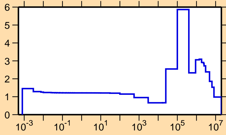
\sigma vs. E for ^{42}\text{Ca}(n,\text{el.})
