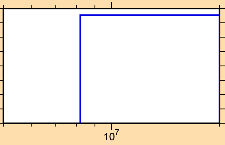
\sigma vs. E for ^{42}\text{Ca}(n,2n)
