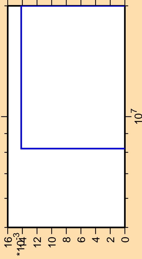
\Delta\sigma/\sigma vs. E for ^{42}\text{Ca} (mt 45)
