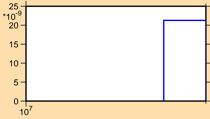
\sigma vs. E for ^{43}\text{Ca}(n,3n)
