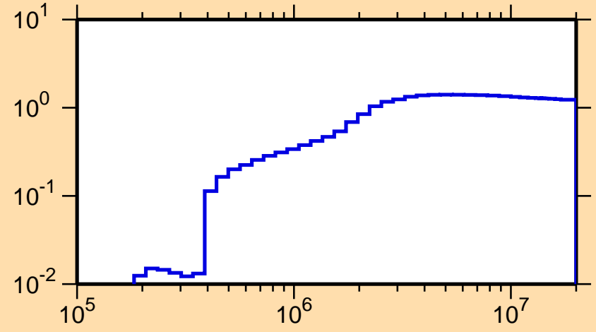
\sigma vs. E for ^{43}\text{Ca}(n,\text{nonel.})
