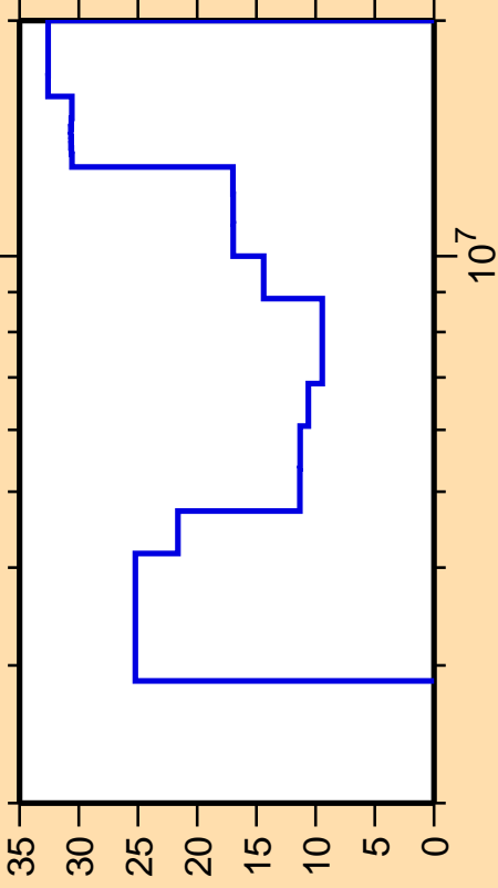
\Delta\sigma/\sigma vs. E for ^{43}\text{Ca}(n,n\text{cont.})
