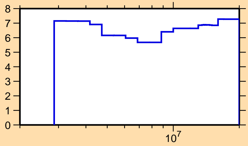
\Delta\sigma/\sigma vs. E for ^{43}\text{Ca}(n,n\text{nonel.})
