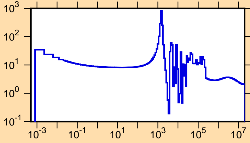
\sigma vs. E for ^{43}\text{Ca}(n,\text{tot.})
