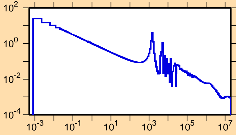
\sigma vs. E for ^{43}\text{Ca}(n,\gamma)
