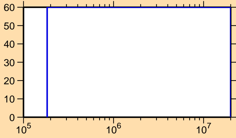
\Delta\sigma/\sigma vs. E for ^{43}\text{Ca}(n,\gamma)
