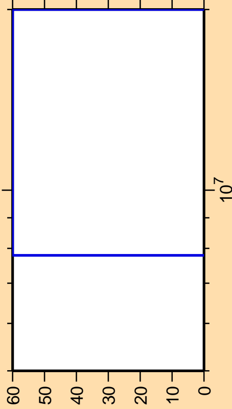
\Delta\sigma/\sigma vs. E for ^{43}\text{Ca}(n,\alpha)
