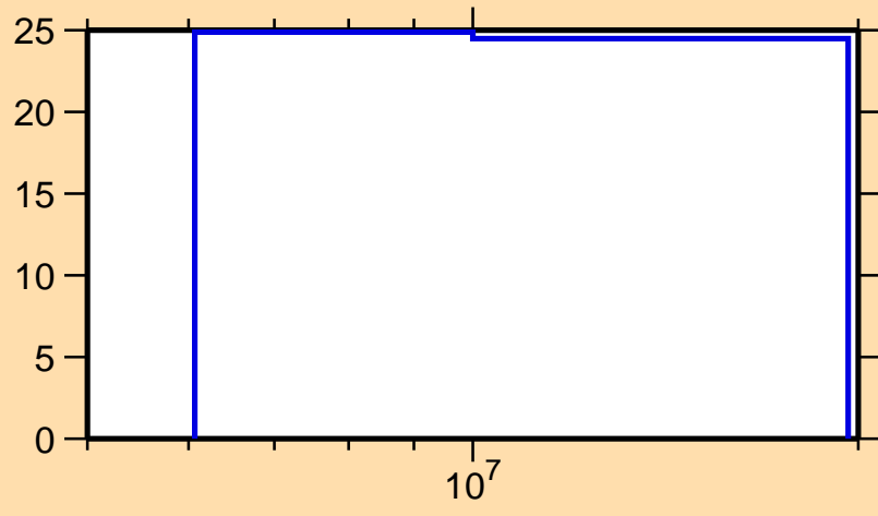
\Delta\sigma/\sigma vs. E for ^{43}\text{Ca}(n,2n)
