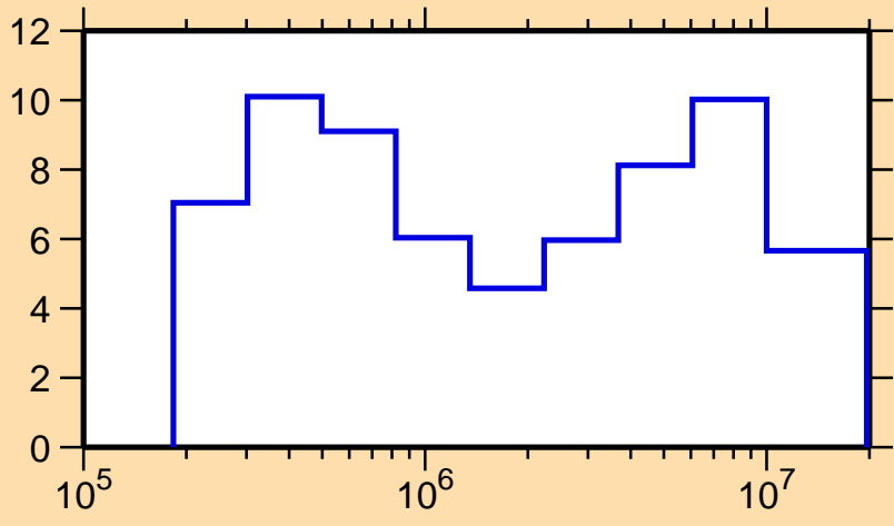
\Delta\sigma/\sigma vs. E for ^{43}\text{Ca}(n,\text{el.})
