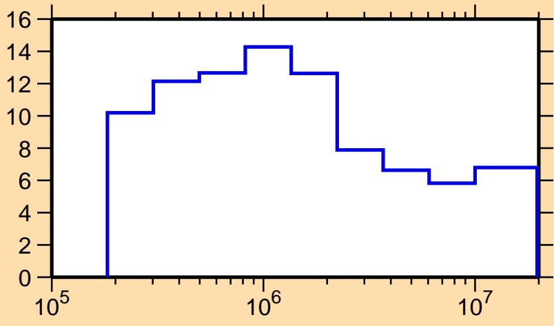
\Delta\sigma/\sigma vs. E for ^{43}\text{Ca}(n,\text{nonel.})
