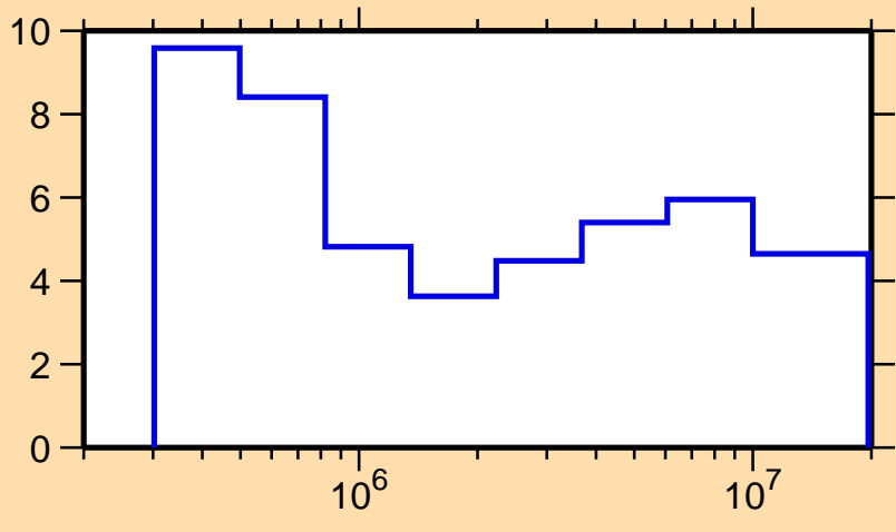
\Delta\sigma/\sigma vs. E for ^{43}\text{Ca}(n,\text{tot.})
