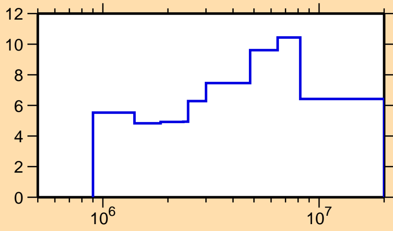
\Delta\sigma/\sigma vs. E for ^{43}\text{Ca}(n,el.)
