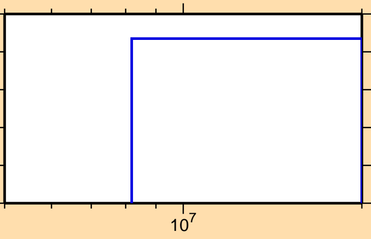
\sigma vs. E for ^{43}\text{Ca}(n,\text{He}3)
