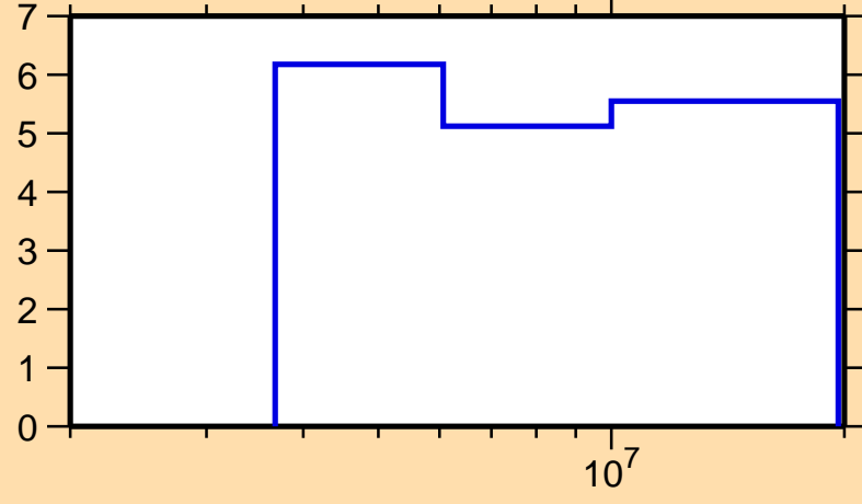
\Delta\sigma/\sigma vs. E for ^{44}\text{Ca}(n,n\text{nonel.})
