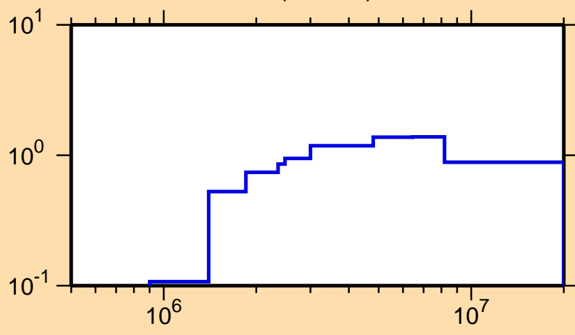
\sigma vs. E for ^{44}\text{Ca}(n,\text{inel.})
