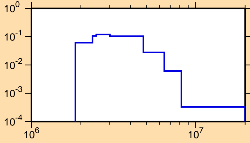
\sigma vs. E for ^{44}\text{Ca}(n,n_2)
