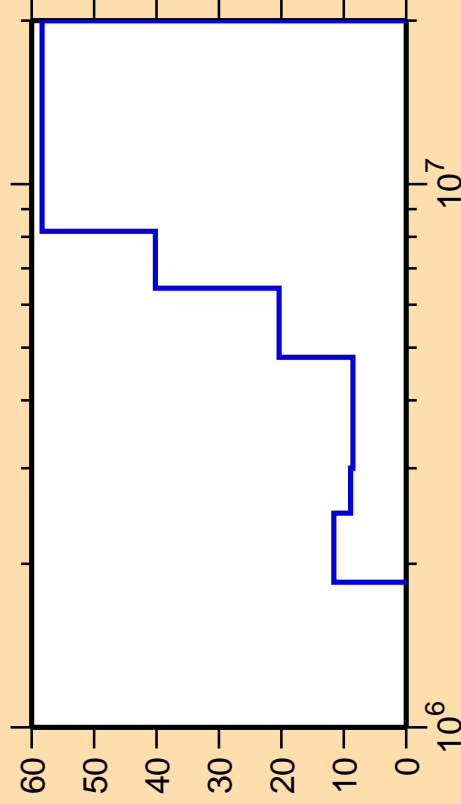
\Delta\sigma/\sigma vs. E for ^{44}\text{Ca}(n,n_2)
