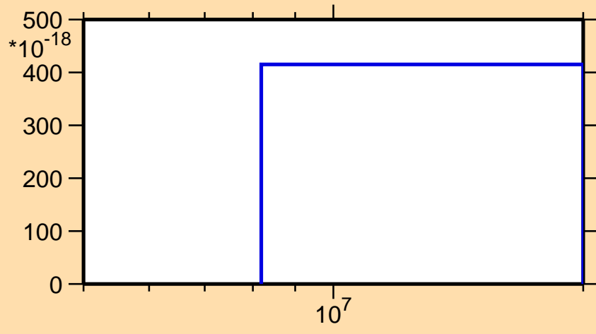
\sigma vs. E for ^{44}\text{Ca}(n,p\alpha)
