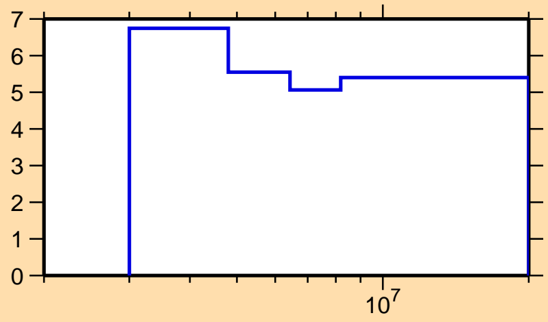
\Delta\sigma/\sigma vs. E for ^{44}\text{Ca}(n,n\text{onel.})
