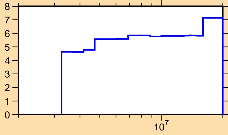
\Delta\sigma/\sigma vs. E for ^{45}\text{Ca}(n,n\text{onel.})
