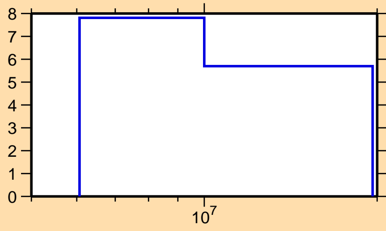
\Delta\sigma/\sigma vs. E for ^{45}\text{Ca}(n,\text{tot.})
