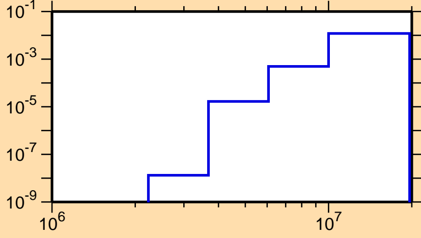
\sigma vs. E for ^{45}\text{Ca}(n,\alpha)
