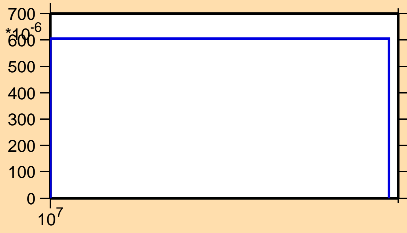
\sigma vs. E for ^{45}\text{Ca}(n,d)
