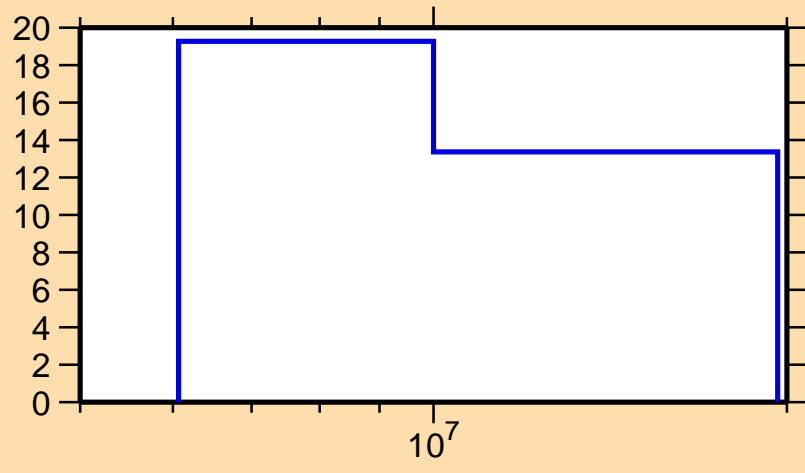
\Delta\sigma/\sigma vs. E for ^{45}\text{Ca}(n,2n)
