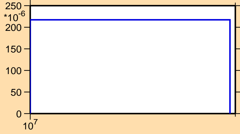
\sigma vs. E for ^{45}\text{Ca}(n,n\alpha)
