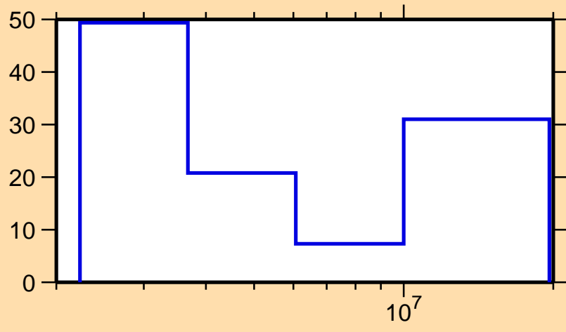
\Delta\sigma/\sigma vs. E for ^{45}\text{Ca}(n,n\text{cont.})
