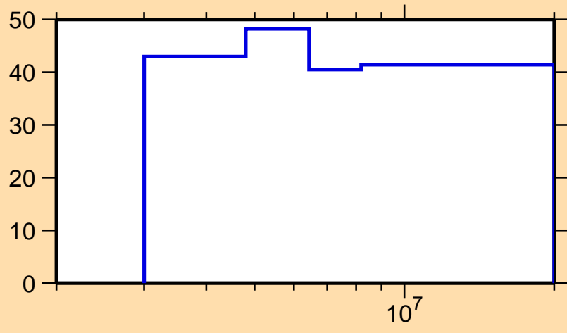
\Delta\sigma/\sigma vs. E for ^{45}\text{Ca}(n,p)
