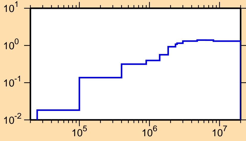
\sigma vs. E for ^{45}\text{Ca}(n,\text{nonel.})
