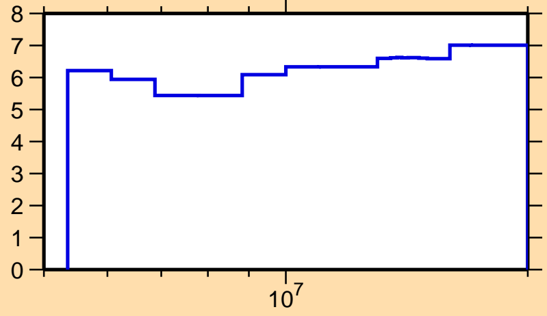
\Delta\sigma/\sigma vs. E for ^{46}\text{Ca}(n,n\text{onel.})
