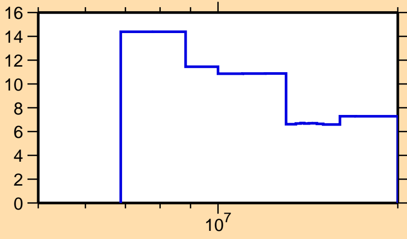
\Delta\sigma/\sigma vs. E for ^{46}\text{Ca}(n,el.)
