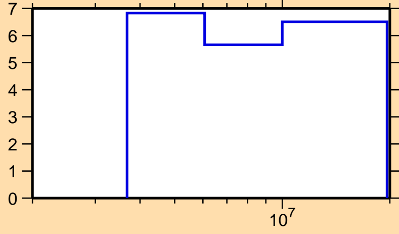
\Delta\sigma/\sigma vs. E for ^{46}\text{Ca}(n,n\text{nonel.})
