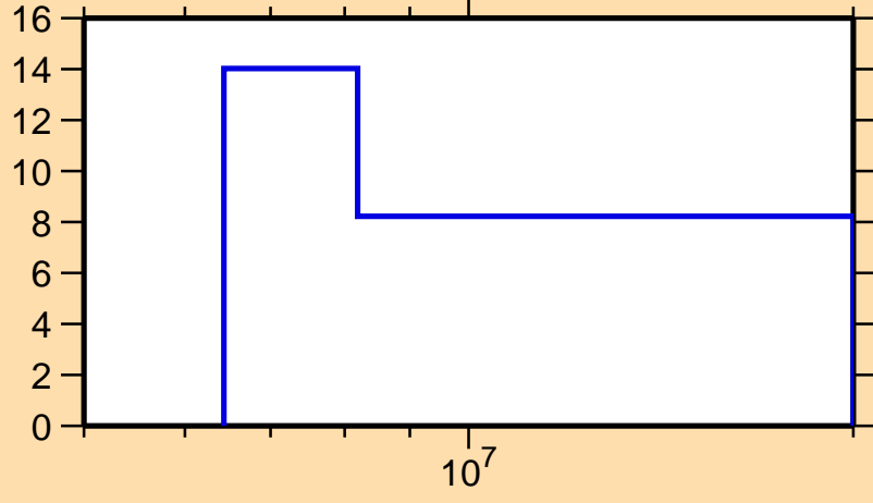
\Delta\sigma/\sigma vs. E for ^{46}\text{Ca}(n,el.)
