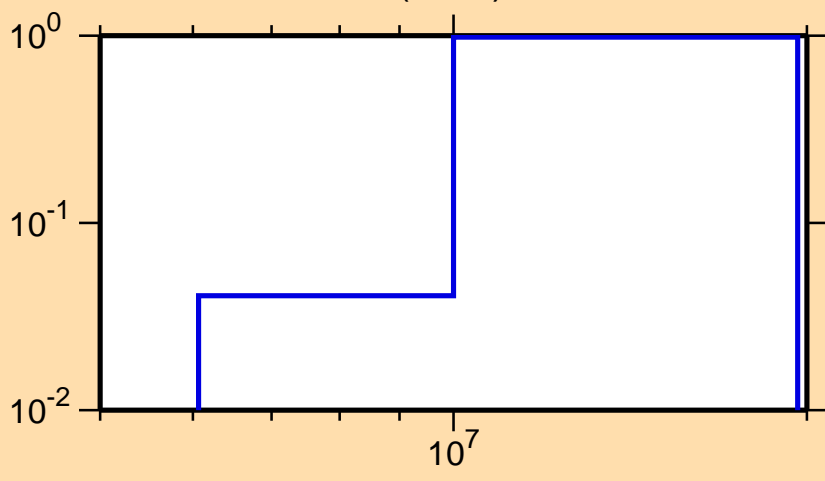
\sigma vs. E for ^{47}\text{Ca}(n,2n)
