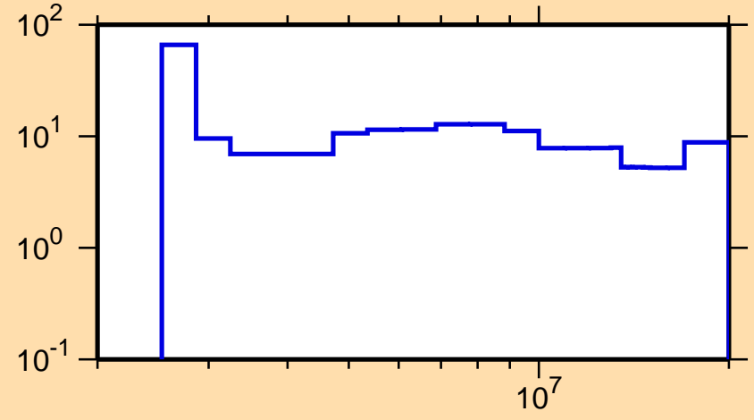
\Delta\sigma/\sigma vs. E for ^{48}\text{Ca}(n,\text{el.})
