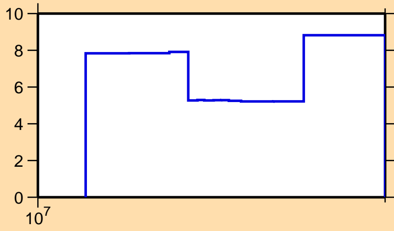
\Delta\sigma/\sigma vs. E for ^{48}\text{Ca}(n,el.)
