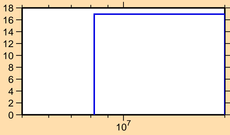
\Delta\sigma/\sigma vs. E for ^{48}\text{Ca}(n,n_1)
