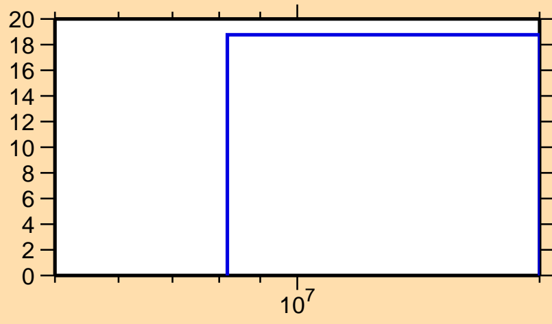
\Delta\sigma/\sigma vs. E for ^{48}\text{Ca}(n,ncont.)
