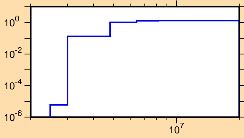
\sigma vs. E for ^{48}\text{Ca}(n,\text{nonel.})
