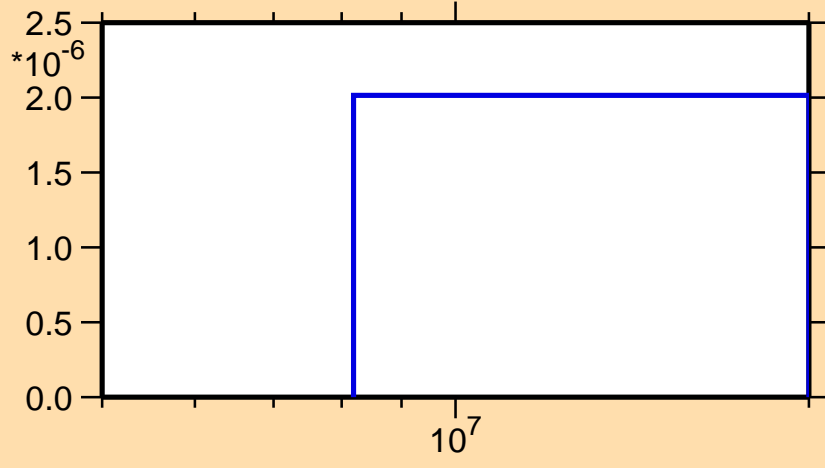
\sigma vs. E for ^{48}\text{Ca}(n,d)
