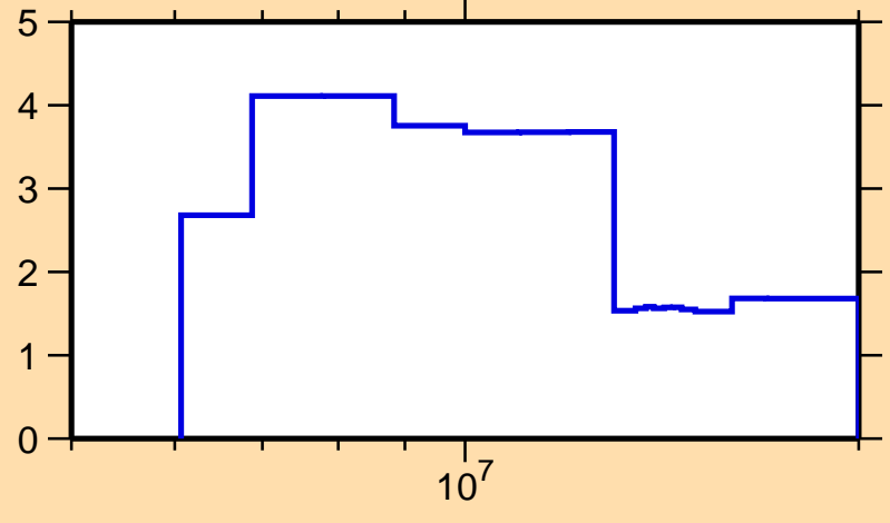
\Delta\sigma/\sigma vs. E for ^{49}\text{Ca}(n,\text{el.})
