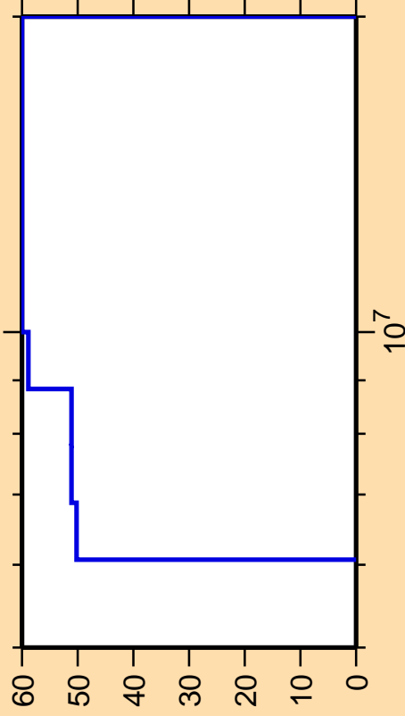
\Delta\sigma/\sigma vs. E for ^{49}\text{Ca}(n,n\text{cont.})
