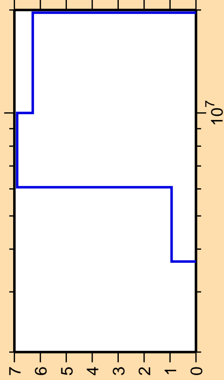
\Delta\sigma/\sigma vs. E for ^{49}\text{Ca}(n,n_4)
