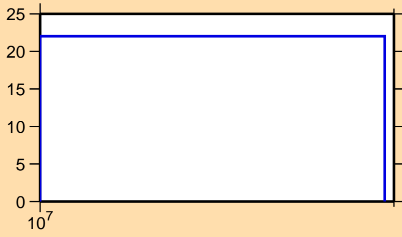
\Delta\sigma/\sigma vs. E for ^{49}\text{Ca}(n,n_1)
