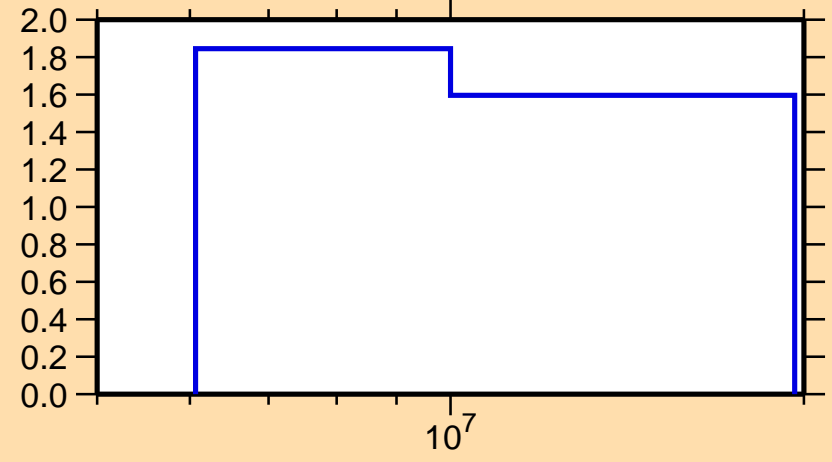
\Delta\sigma/\sigma vs. E for ^{49}\text{Ca}(n,n\text{onel.})
