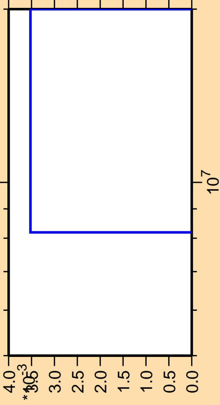
\Delta\sigma/\sigma vs. E for ^{49}\text{Ca}(n,\text{nd})
