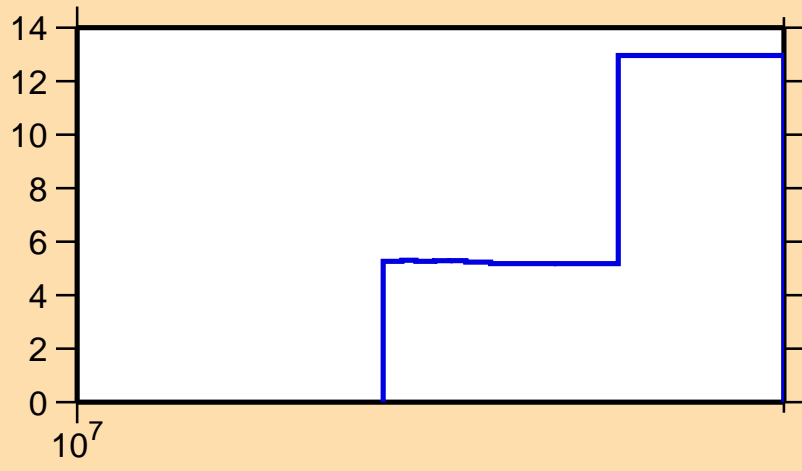
\Delta\sigma/\sigma vs. E for ^{50}\text{Ca}(n,el.)
