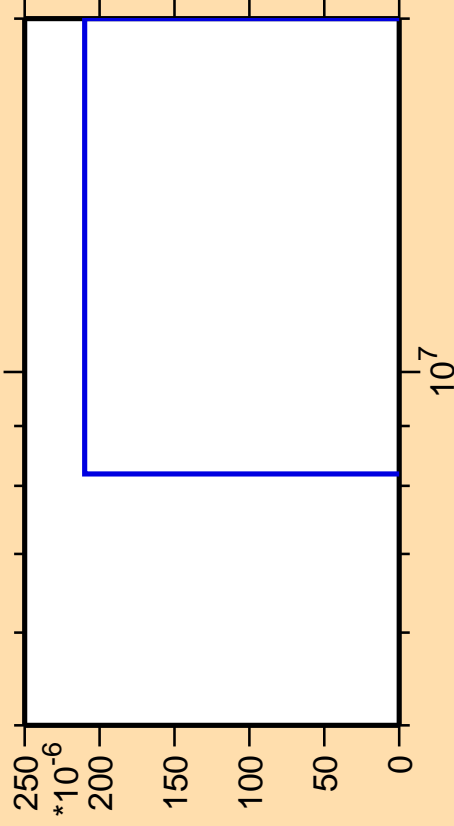
\Delta\sigma/\sigma vs. E for ^{50}\text{Ca}(n,nt)
