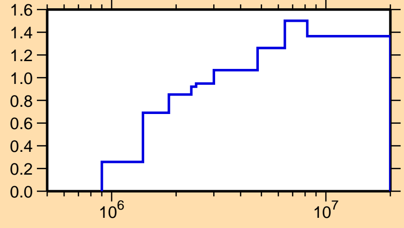
\sigma vs. E for ^{50}\text{Ca}(n,\text{nonel.})
