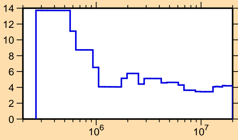
\Delta\sigma/\sigma vs. E for ^{97}\text{Cd}(n,n\text{nonel.})
