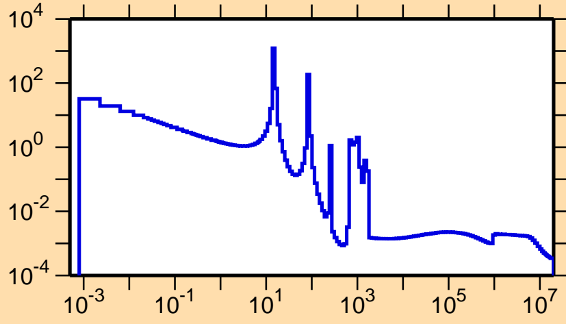
\sigma vs. E for ^{97}\text{Cd}(n,\gamma)
