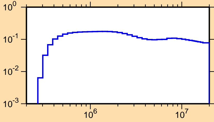
\sigma vs. E for ^{97}\text{Cd}(n,\text{inel.})
