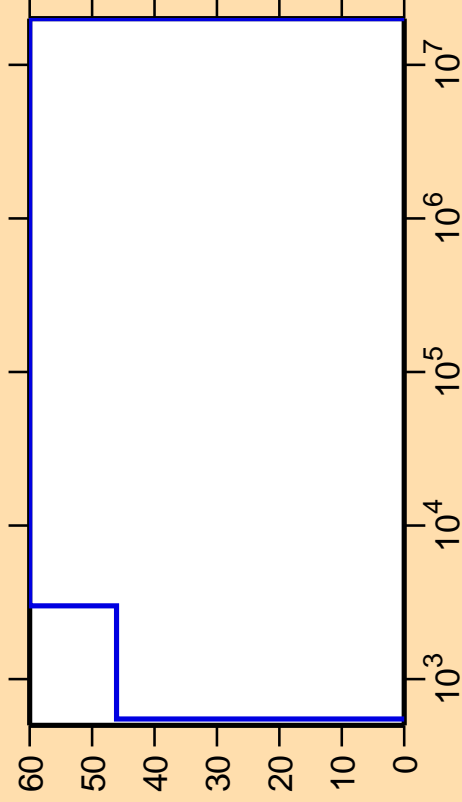
\Delta\sigma/\sigma vs. E for ^{97}\text{Cd}(n,p\alpha)
