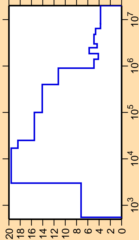
\Delta\sigma/\sigma vs. E for ^{97}\text{Cd}(n,\text{nonel.})
