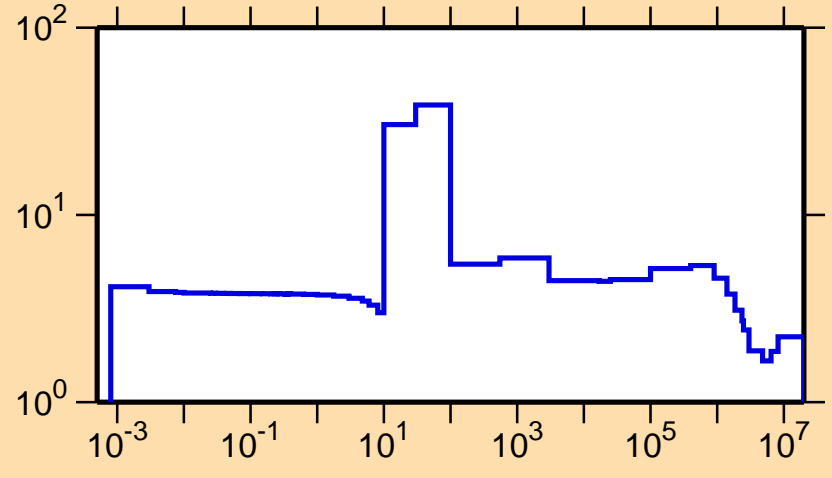
\sigma vs. E for ^{97}\text{Cd}(n,\text{el.})
