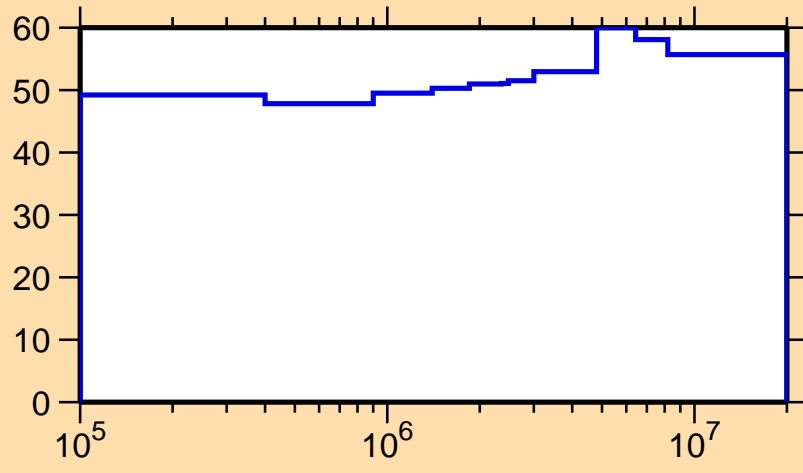
\Delta\sigma/\sigma vs. E for ^{97}\text{Cd}(n,ncont.)
