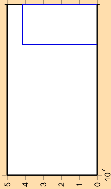
\Delta\sigma/\sigma vs. E for ^{98}\text{Cd}(n,2np)
