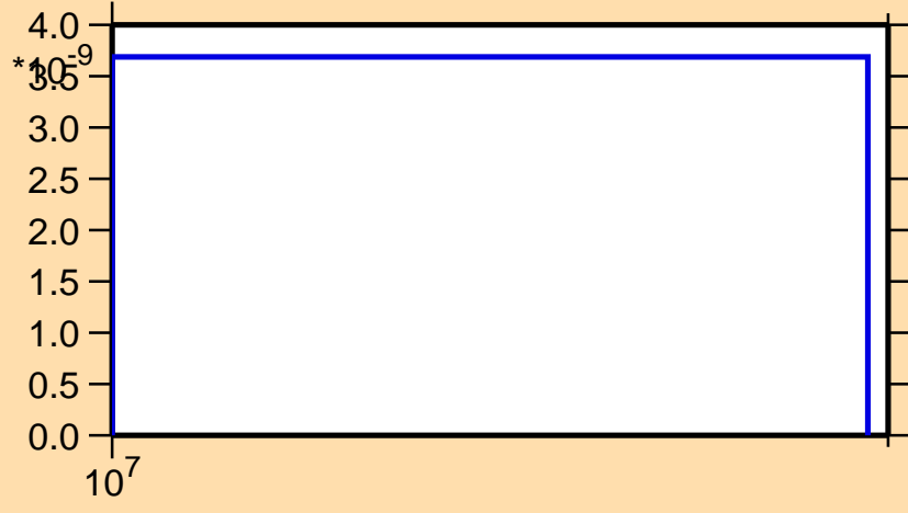
\sigma vs. E for ^{98}\text{Cd}(n,\text{pt})
