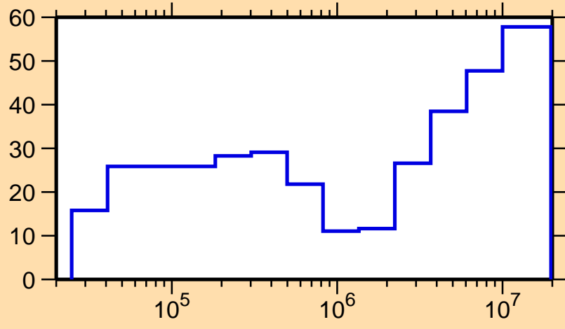
\Delta\sigma/\sigma vs. E for ^{98}\text{Cd}(n,p)
