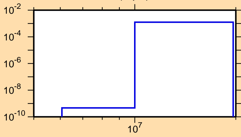
\sigma vs. E for ^{98}\text{Cd}(n,\text{pd})
