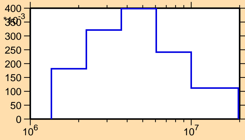
\sigma vs. E for ^{98}\text{Cd}(n,\text{inel.})
