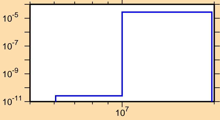
\sigma vs. E for ^{98}\text{Cd}(n,n\alpha)
