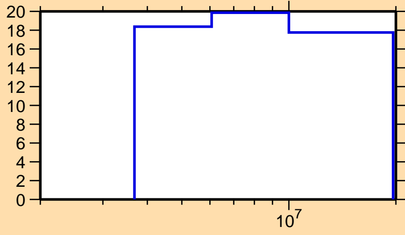
\Delta\sigma/\sigma vs. E for ^{98}\text{Cd}(n,n\text{nonel.})
