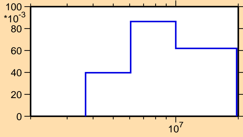
\sigma vs. E for ^{98}\text{Cd}(n,n\text{cont.})
