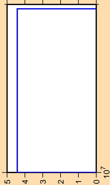
\Delta\sigma/\sigma vs. E for ^{98}\text{Cd}(\text{mt117})
