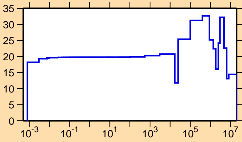
\Delta\sigma/\sigma vs. E for ^{98}\text{Cd}(n,\text{el.})
