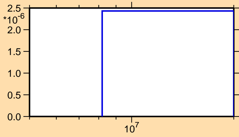
\sigma vs. E for ^{98}\text{Cd}(n,t)
