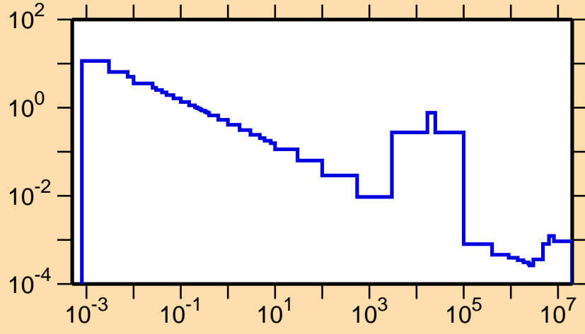
\sigma vs. E for ^{98}\text{Cd}(n,\gamma)
