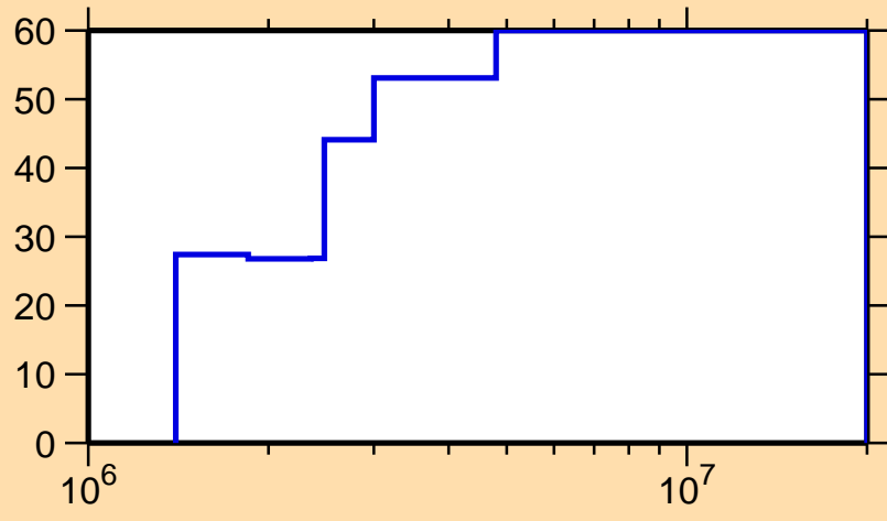
\Delta\sigma/\sigma vs. E for ^{98}\text{Cd}(n,n_1)
