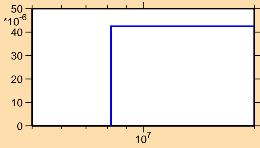
\sigma vs. E for ^{98}\text{Cd}(n,2n)
