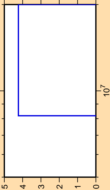
\Delta\sigma/\sigma vs. E for ^{98}\text{Cd}(\text{mt117})
