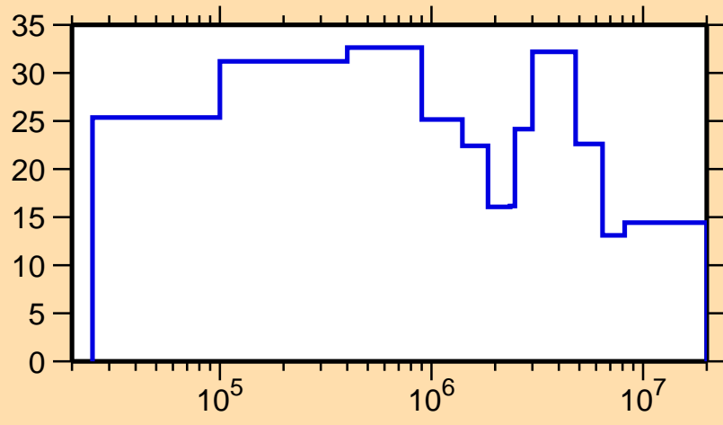
\Delta\sigma/\sigma vs. E for ^{98}\text{Cd}(n,el.)
