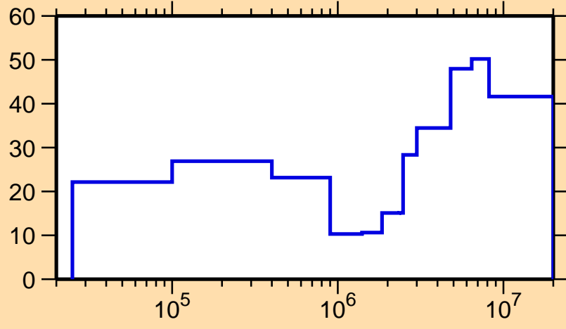
\Delta\sigma/\sigma vs. E for ^{98}\text{Cd}(n,p)
