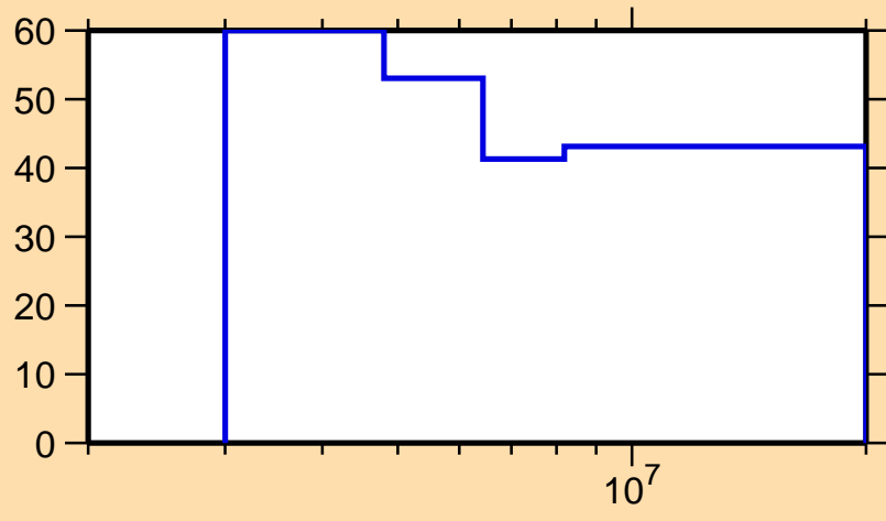
\Delta\sigma/\sigma vs. E for ^{98}\text{Cd}(n,n\text{cont.})
