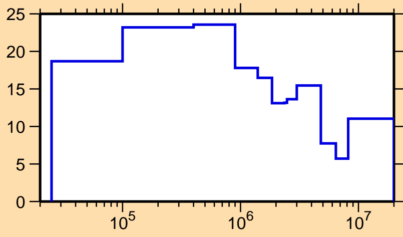
\Delta\sigma/\sigma vs. E for ^{98}\text{Cd}(n,\text{tot.})
