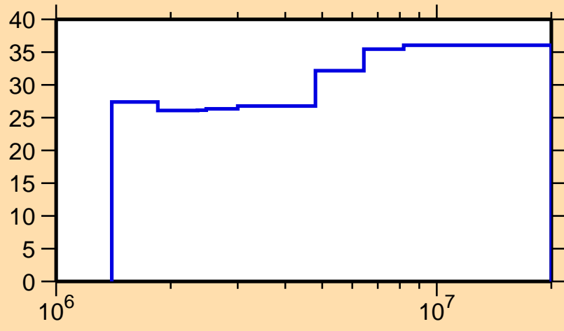
\Delta\sigma/\sigma vs. E for ^{98}\text{Cd}(n,\text{inel.})
