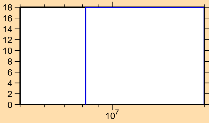
\Delta\sigma/\sigma vs. E for ^{98}\text{Cd}(n,\text{nonel.})
