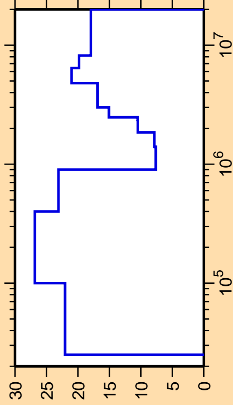
\Delta\sigma/\sigma vs. E for ^{98}\text{Cd}(n,\text{nonel.})
