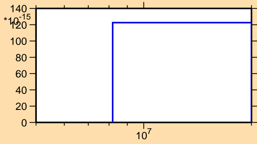
\sigma vs. E for ^{98}\text{Cd}(n,\text{nd})
