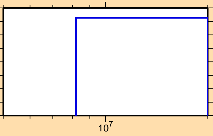
\sigma vs. E for ^{98}\text{Cd}(n,2np)
