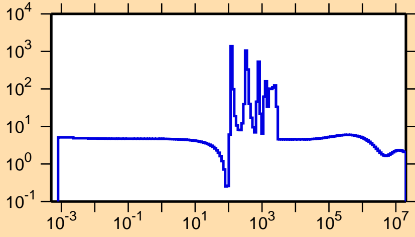
\sigma vs. E for ^{99}\text{Cd}(n,\text{el.})
