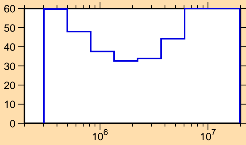
\Delta\sigma/\sigma vs. E for ^{99}\text{Cd}(n,n_1)
