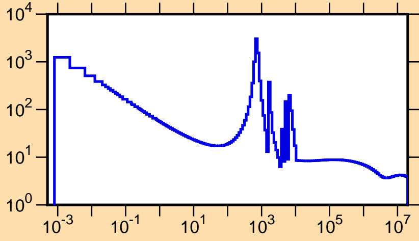
\sigma vs. E for ^{100}\text{Cd}(n,\text{tot.})
