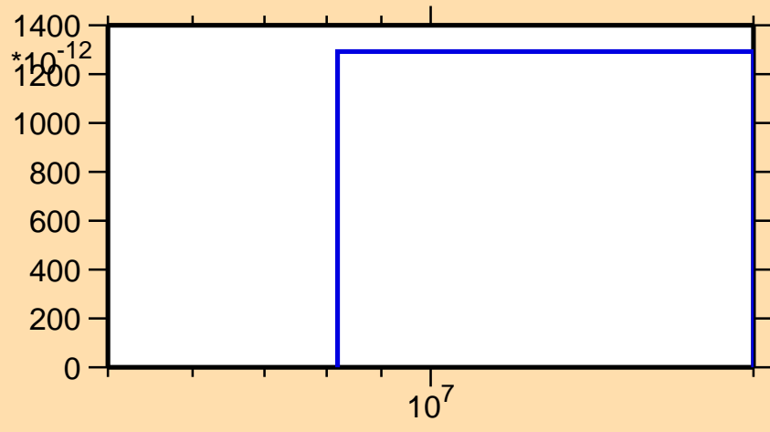
\sigma vs. E for ^{100}\text{Cd}(n,\text{nd})
