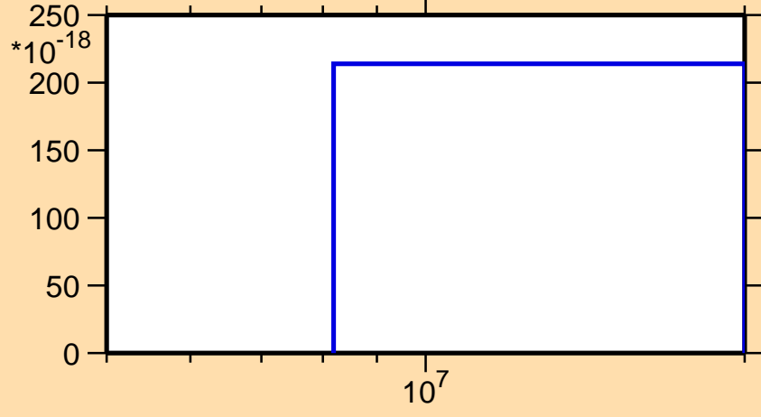
\sigma vs. E for ^{100}\text{Cd}(n,2n\alpha)
