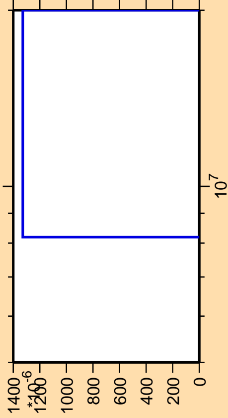
\Delta\sigma/\sigma vs. E for ^{100}\text{Cd}(n,2n\alpha)
