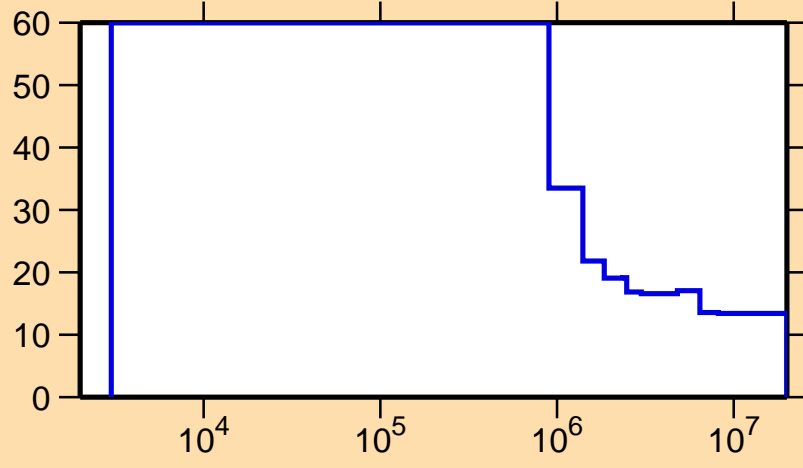
\Delta\sigma/\sigma vs. E for ^{100}\text{Cd}(n,\text{nonel.})
