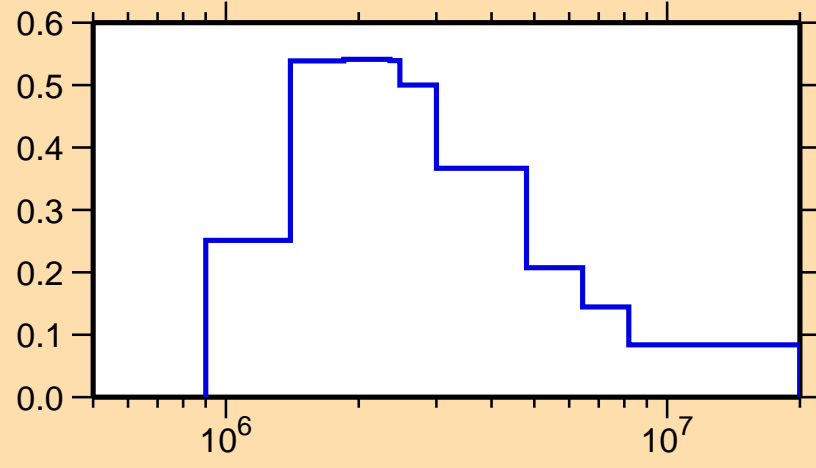
\sigma vs. E for ^{100}\text{Cd}(n,\text{inel.})
