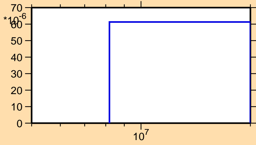
\sigma vs. E for ^{100}\text{Cd}(n,t)
