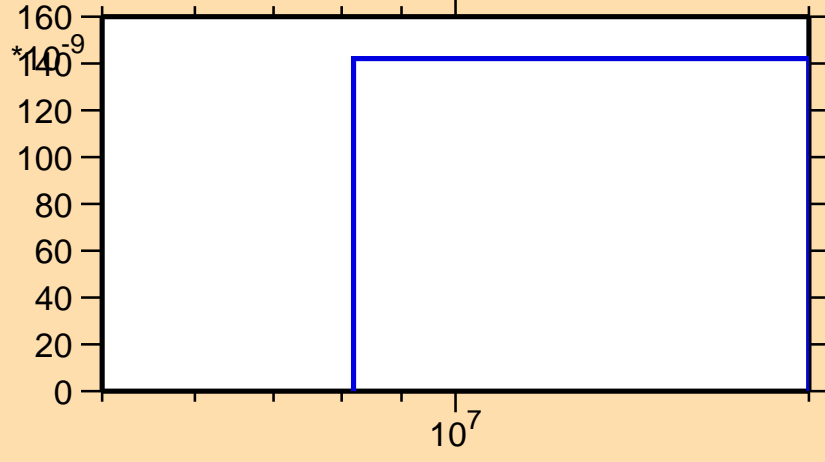
\sigma vs. E for ^{100}\text{Cd}(\text{mt117})
