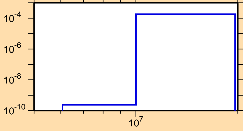
\sigma vs. E for ^{101}\text{Cd}(n,t)
