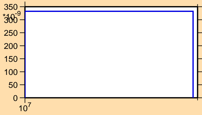
\sigma vs. E for ^{101}\text{Cd}(n,\text{nd})
