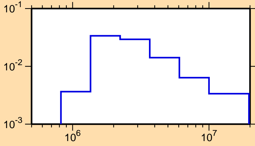
\sigma vs. E for ^{101}\text{Cd}(n,n_3)
