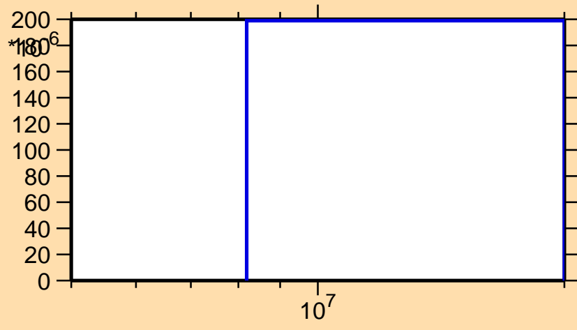
\sigma vs. E for ^{101}\text{Cd}(n,\text{pd})
