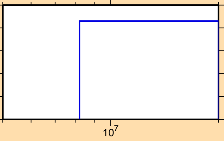
\sigma vs. E for ^{101}\text{Cd}(n,2n\alpha)
