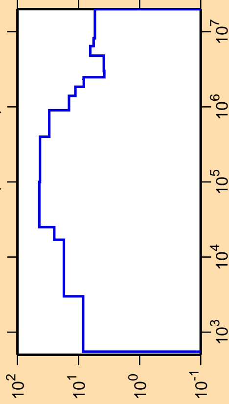
\Delta\sigma/\sigma vs. E for ^{101}\text{Cd}(n,\text{nonel.})
