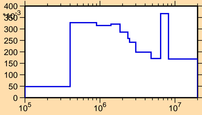
\sigma vs. E for ^{101}\text{Cd}(n,\text{inel.})
