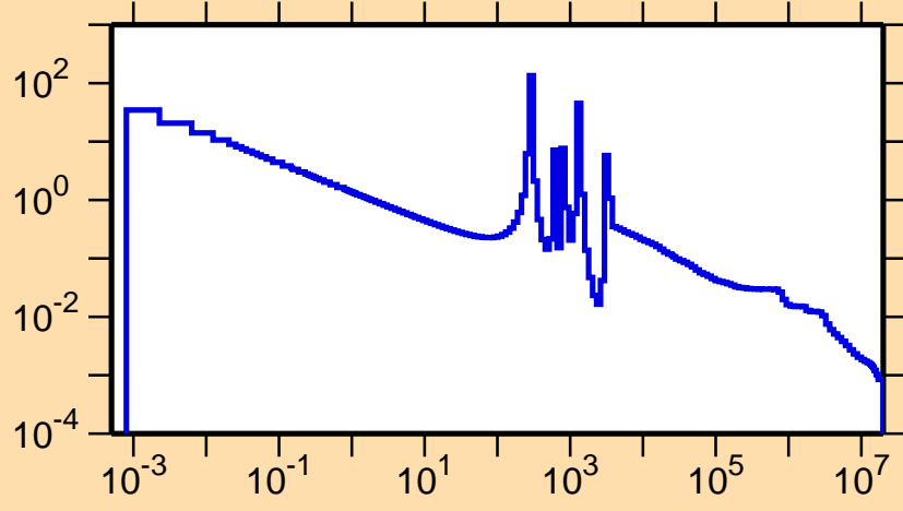
\sigma vs. E for ^{102}\text{Cd}(n,\gamma)
