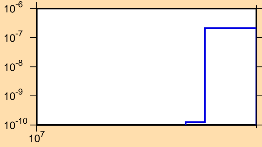
\sigma vs. E for ^{102}\text{Cd}(n,\text{pt})
