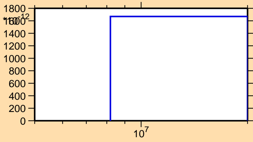
\sigma vs. E for ^{102}\text{Cd}(n,2n\alpha)
