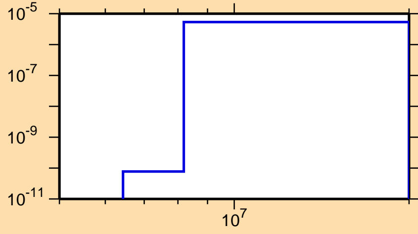
\sigma vs. E for ^{102}\text{Cd}(n,\text{He}3)
