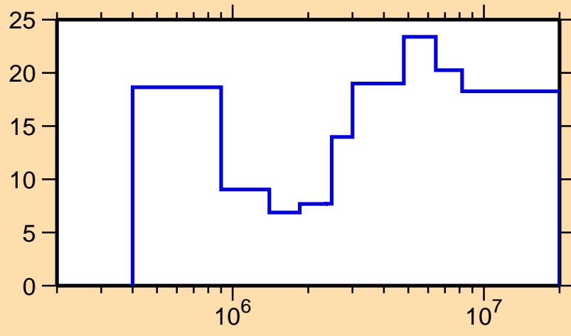
\Delta\sigma/\sigma vs. E for ^{102}\text{Cd}(n,n_1)
