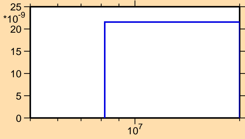
\sigma vs. E for ^{102}\text{Cd}(\text{mt117})
