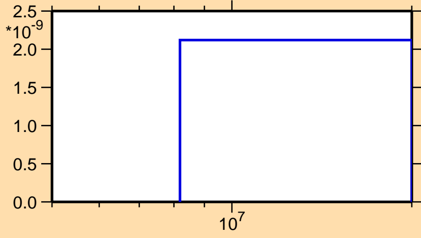
\sigma vs. E for ^{102}\text{Cd}(n,\text{nd})
