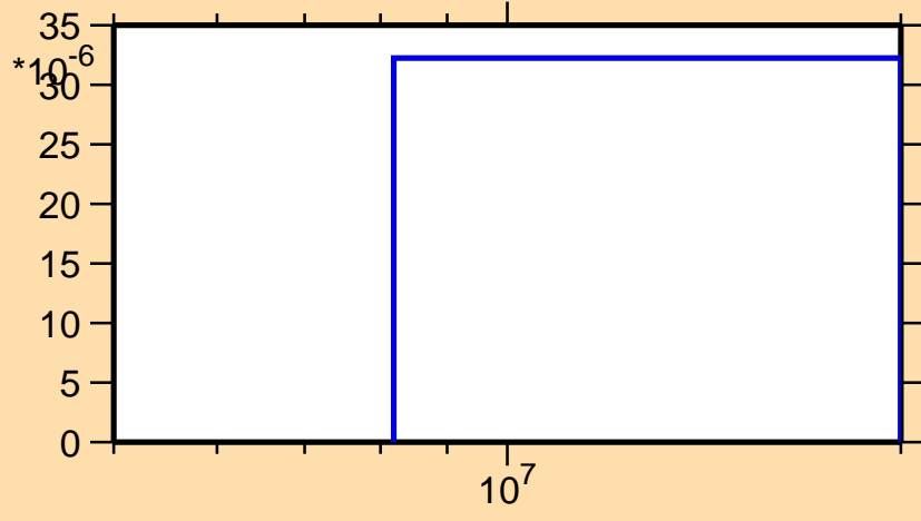
\sigma vs. E for ^{102}\text{Cd}(n,t)
