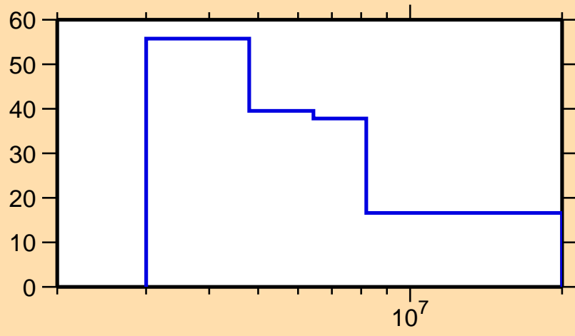
\Delta\sigma/\sigma vs. E for ^{102}\text{Cd}(n,n\text{cont.})
