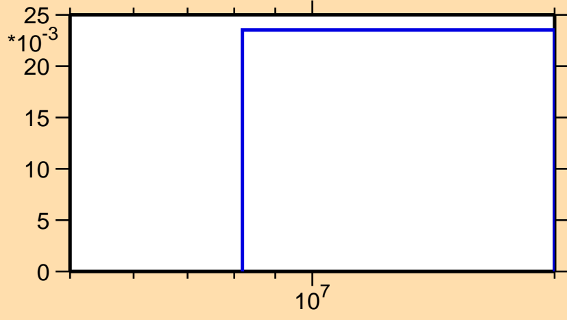
\sigma vs. E for ^{102}\text{Cd}(n,2n)
