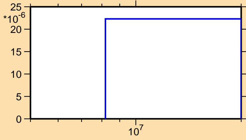
\sigma vs. E for ^{102}\text{Cd}(n,\text{pd})
