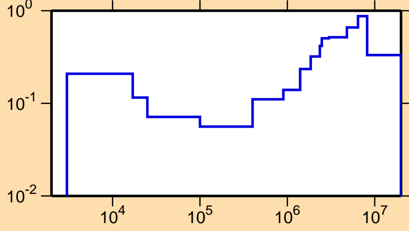
\sigma vs. E for ^{102}\text{Cd}(n,p)
