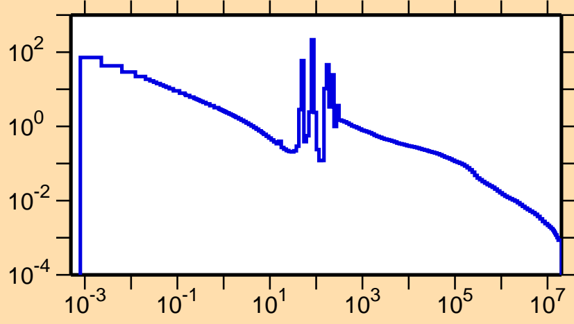
\sigma vs. E for ^{103}\text{Cd}(n,\gamma)
