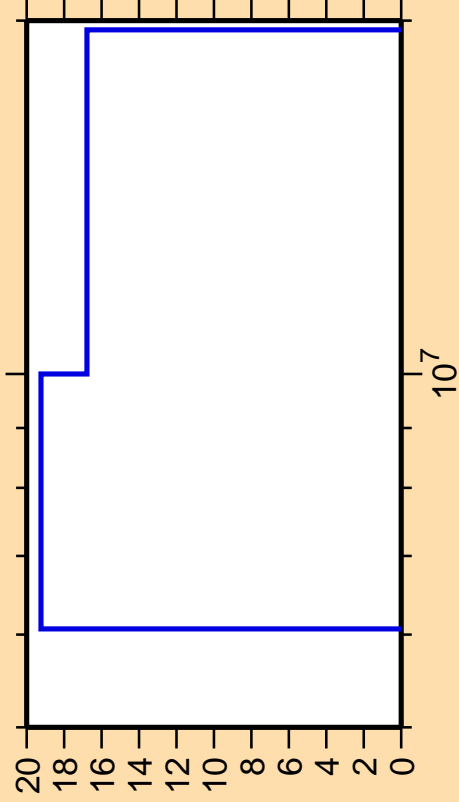
\Delta\sigma/\sigma vs. E for ^{103}\text{Cd}(n,np)
