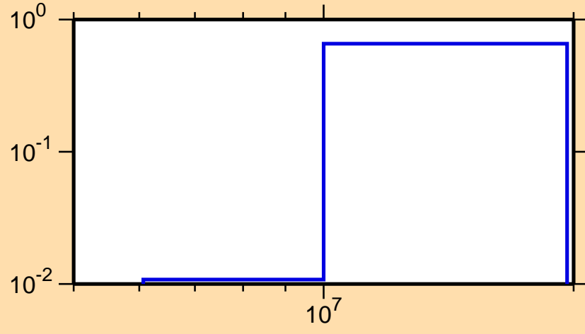
\sigma vs. E for ^{103}\text{Cd}(n,np)
