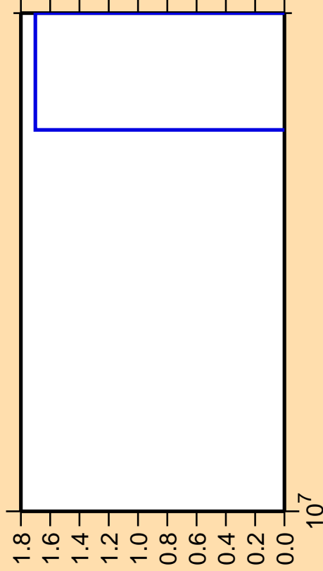
\Delta\sigma/\sigma vs. E for ^{106}\text{Cd}(n,nt)
