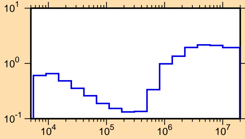
\sigma vs. E for ^{106}\text{Cd}(n,\text{nonel.})
