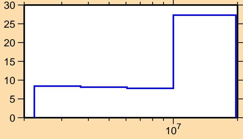
\Delta\sigma/\sigma vs. E for ^{106}\text{Cd}(n,n\text{cont.})
