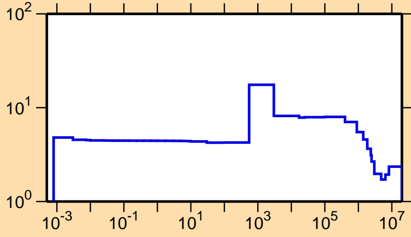
\sigma vs. E for ^{106}\text{Cd}(n,\text{el.})
