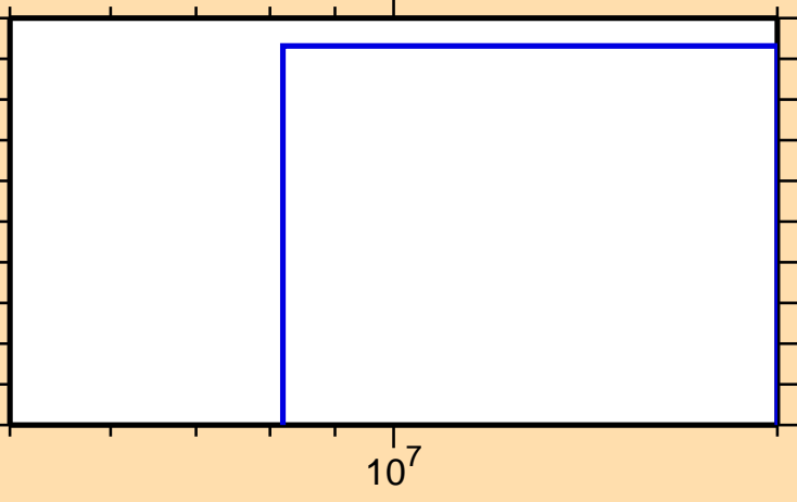
\sigma vs. E for ^{106}\text{Cd}(n,3n)
