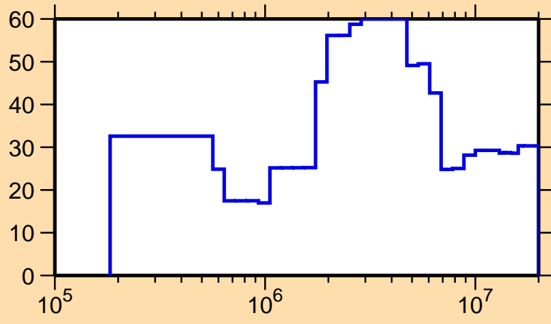
\Delta\sigma/\sigma vs. E for ^{107}\text{Cd}(n,n_1)
