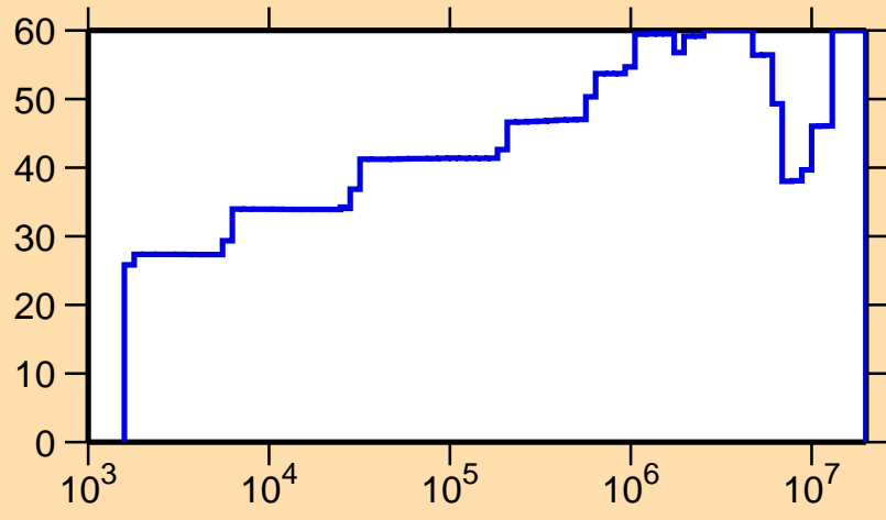
\Delta\sigma/\sigma vs. E for ^{107}\text{Cd}(n,\gamma)
