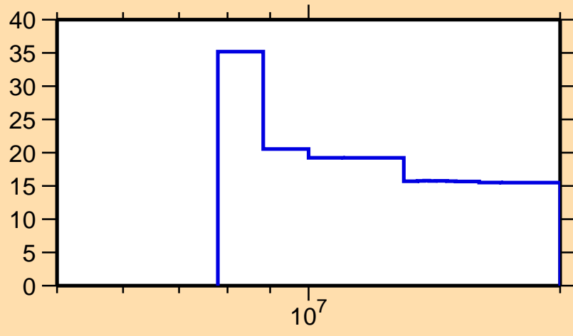
\Delta\sigma/\sigma vs. E for ^{107}\text{Cd}(n,2n)
