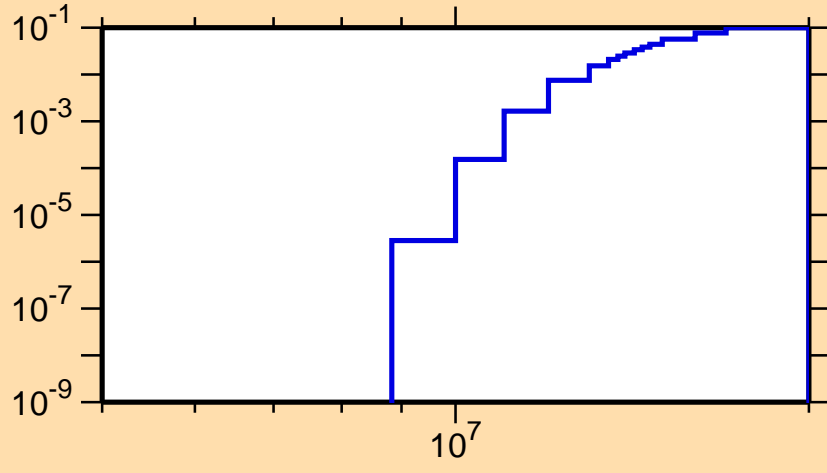
\sigma vs. E for ^{107}\text{Cd}(n,np)
