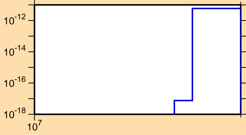
\sigma vs. E for ^{107}\text{Cd}(n,nt)
