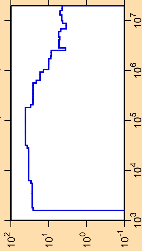
\Delta\sigma/\sigma vs. E for ^{107}\text{Cd}(n,\text{nonel.})
