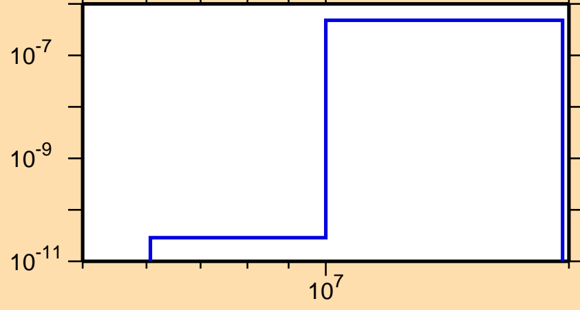
\sigma vs. E for ^{107}\text{Cd}(n,p\alpha)
